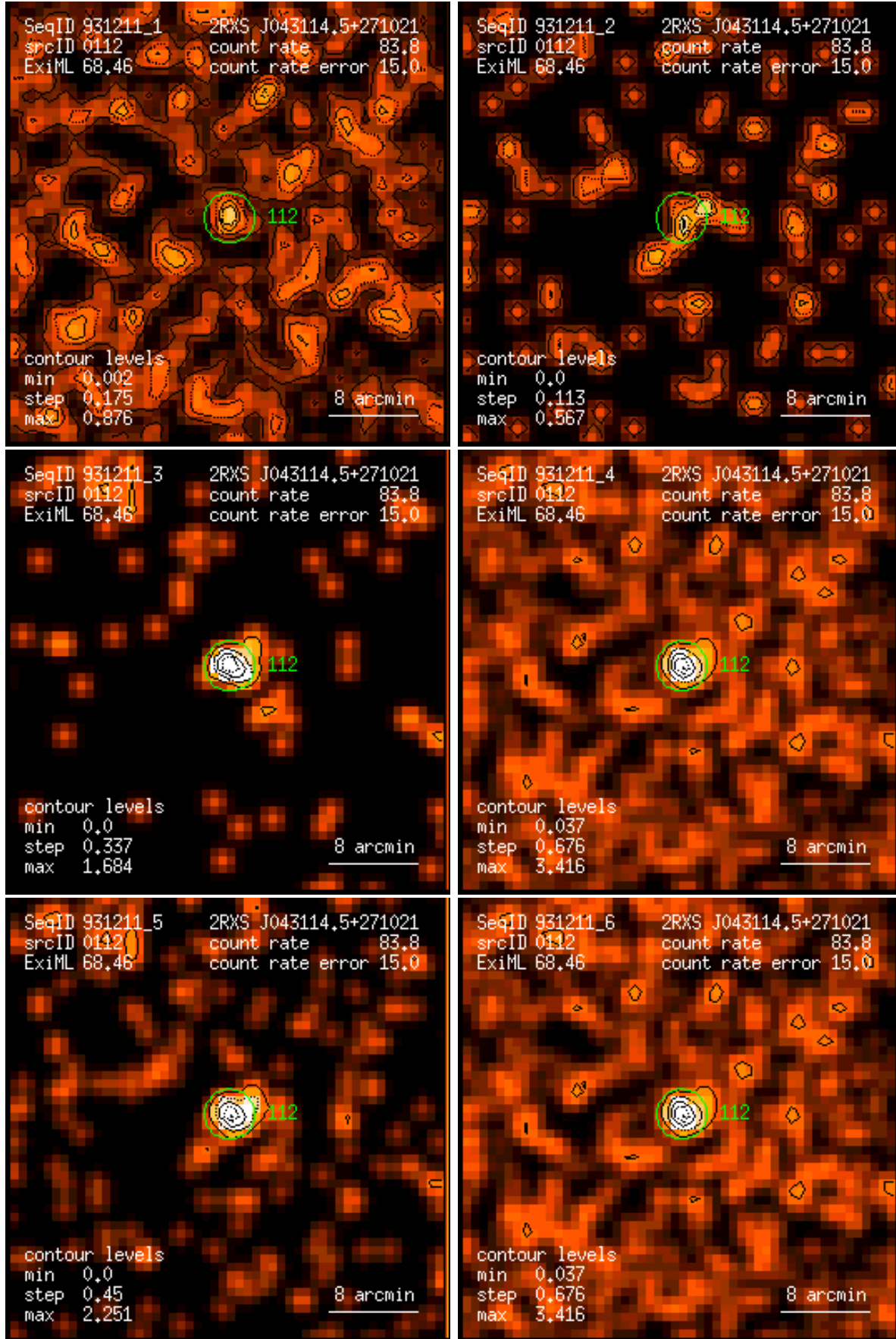
Figure 112: RASS 931211: detection 0112: band rate images, Gaussian filter: (1) PSPC channels 11 – 41, (2) 52 – 90, (3) 91 – 201, (4) 11 – 235, (5) 52 – 201, (6) 11 – 201. Broad band rates in counts/ks. Band rate contour levels in counts/ks/arcmin 2 .
