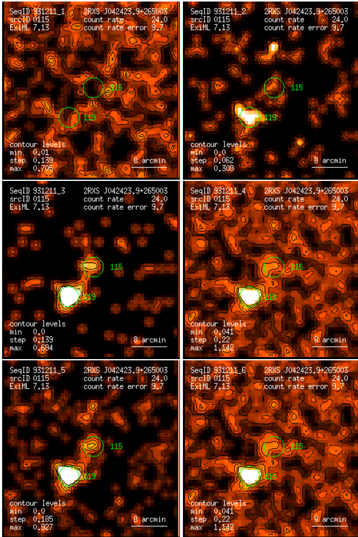
Figure 115: RASS 931211: detection 0115: band rate images, Gaussian filter: (1) PSPC channels 11 – 41, (2) 52 – 90, (3) 91 – 201, (4) 11 – 235, (5) 52 – 201, (6) 11 – 201. Broad band rates in counts/ks. Band rate contour levels in counts/ks/arcmin 2 .
