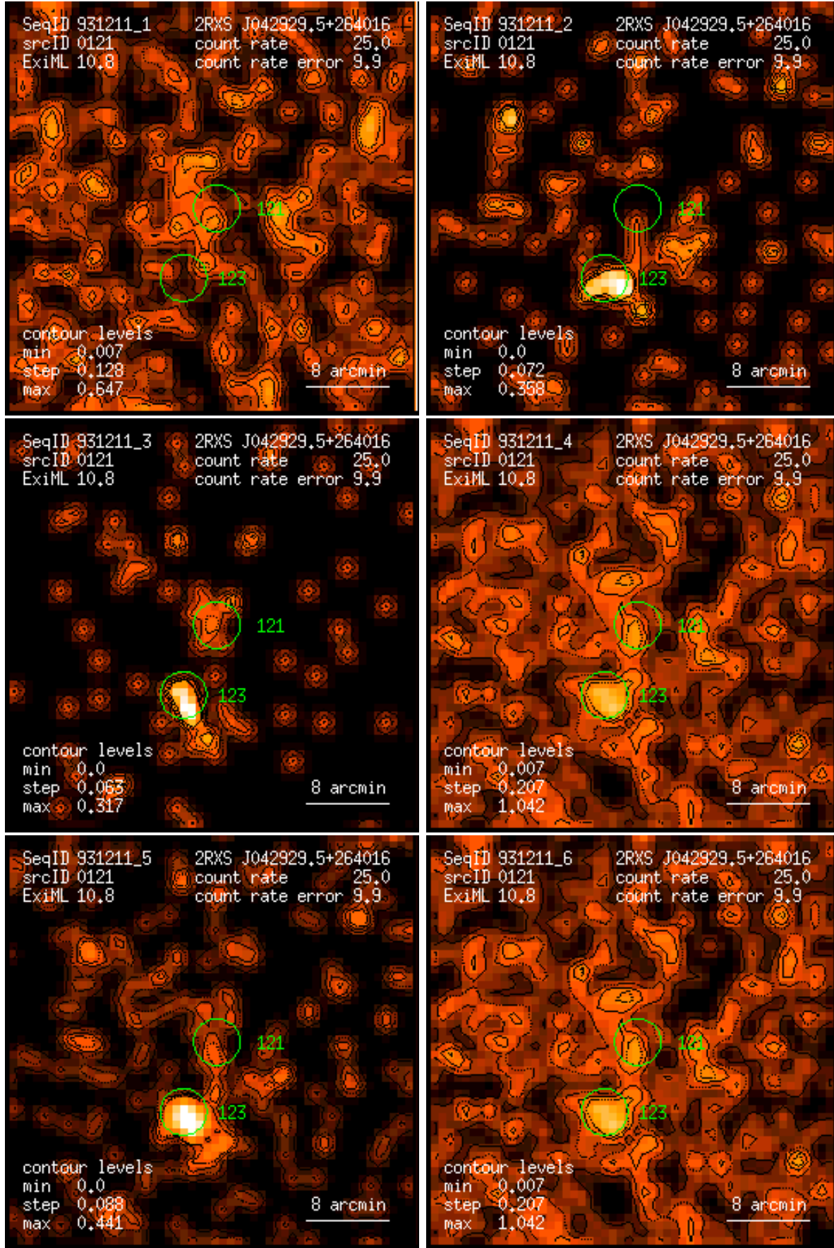
Figure 121: RASS 931211: detection 0121: band rate images, Gaussian filter: (1) PSPC channels 11 – 41, (2) 52 – 90, (3) 91 – 201, (4) 11 – 235, (5) 52 – 201, (6) 11 – 201. Broad band rates in counts/ks. Band rate contour levels in counts/ks/arcmin 2 .
