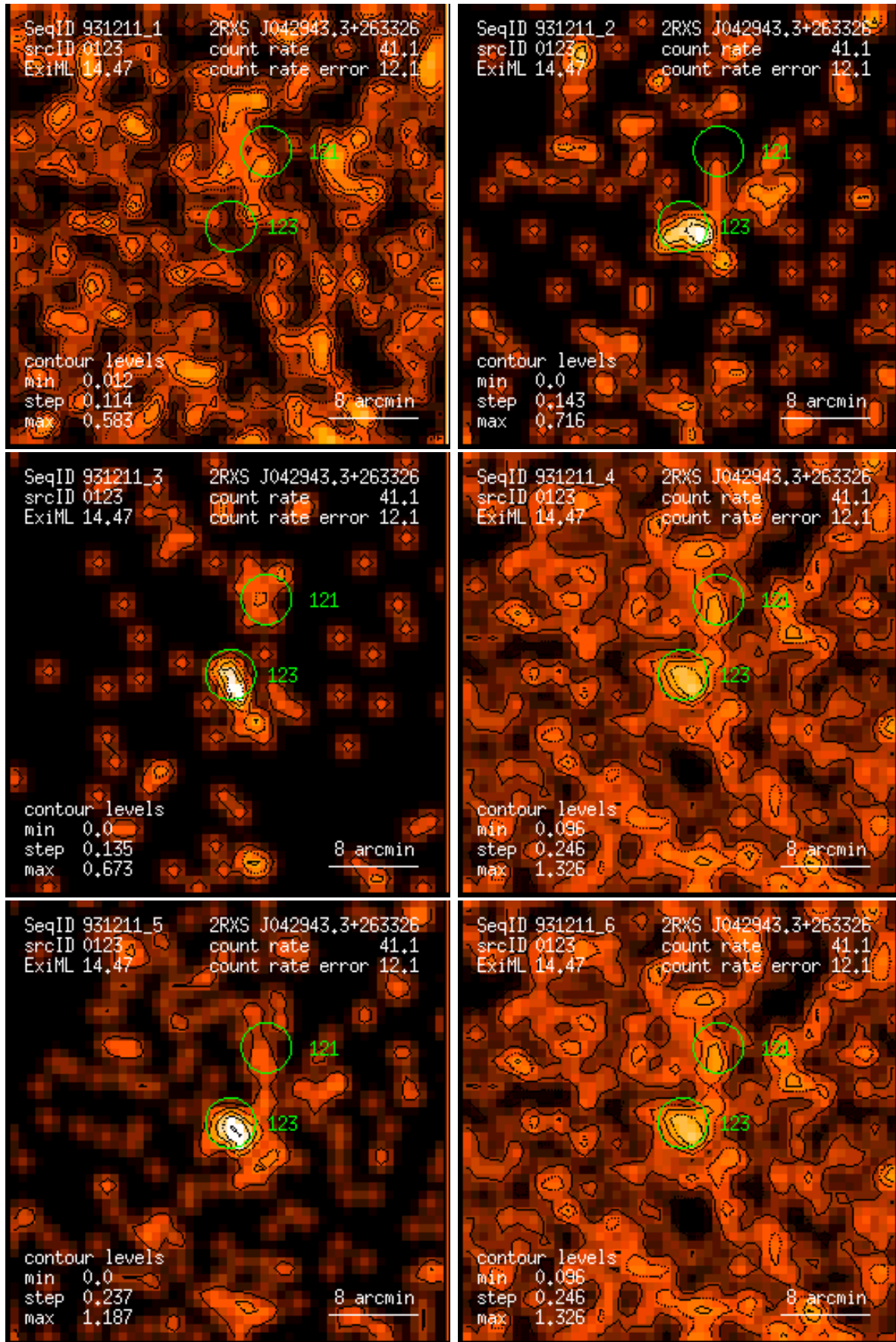
Figure 123: RASS 931211: detection 0123: band rate images, Gaussian filter: (1) PSPC channels 11 – 41, (2) 52 – 90, (3) 91 – 201, (4) 11 – 235, (5) 52 – 201, (6) 11 – 201. Broad band rates in counts/ks. Band rate contour levels in counts/ks/arcmin 2 .
