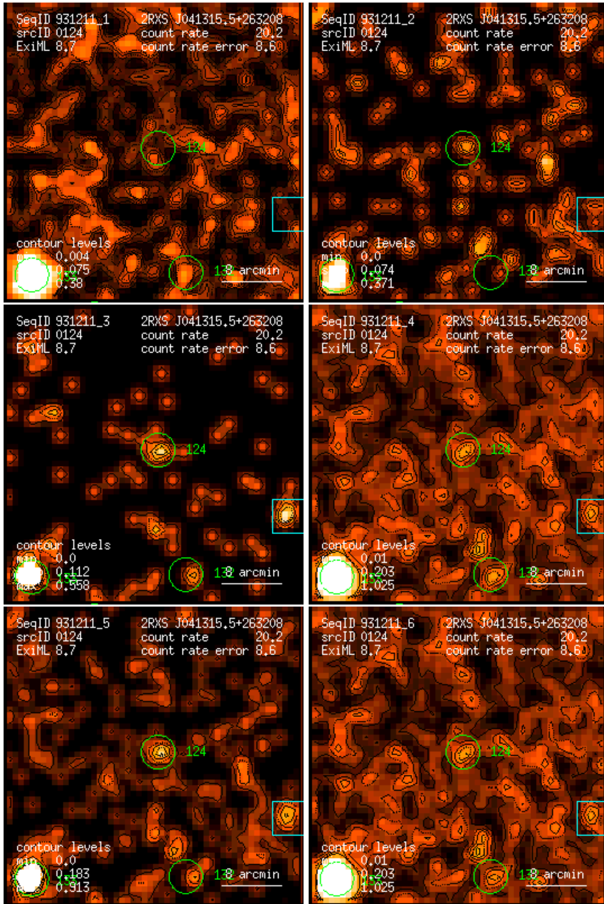
Figure 124: RASS 931211: detection 0124: band rate images, Gaussian filter: (1) PSPC channels 11 – 41, (2) 52 – 90, (3) 91 – 201, (4) 11 – 235, (5) 52 – 201, (6) 11 – 201. Broad band rates in counts/ks. Band rate contour levels in counts/ks/arcmin 2 .
