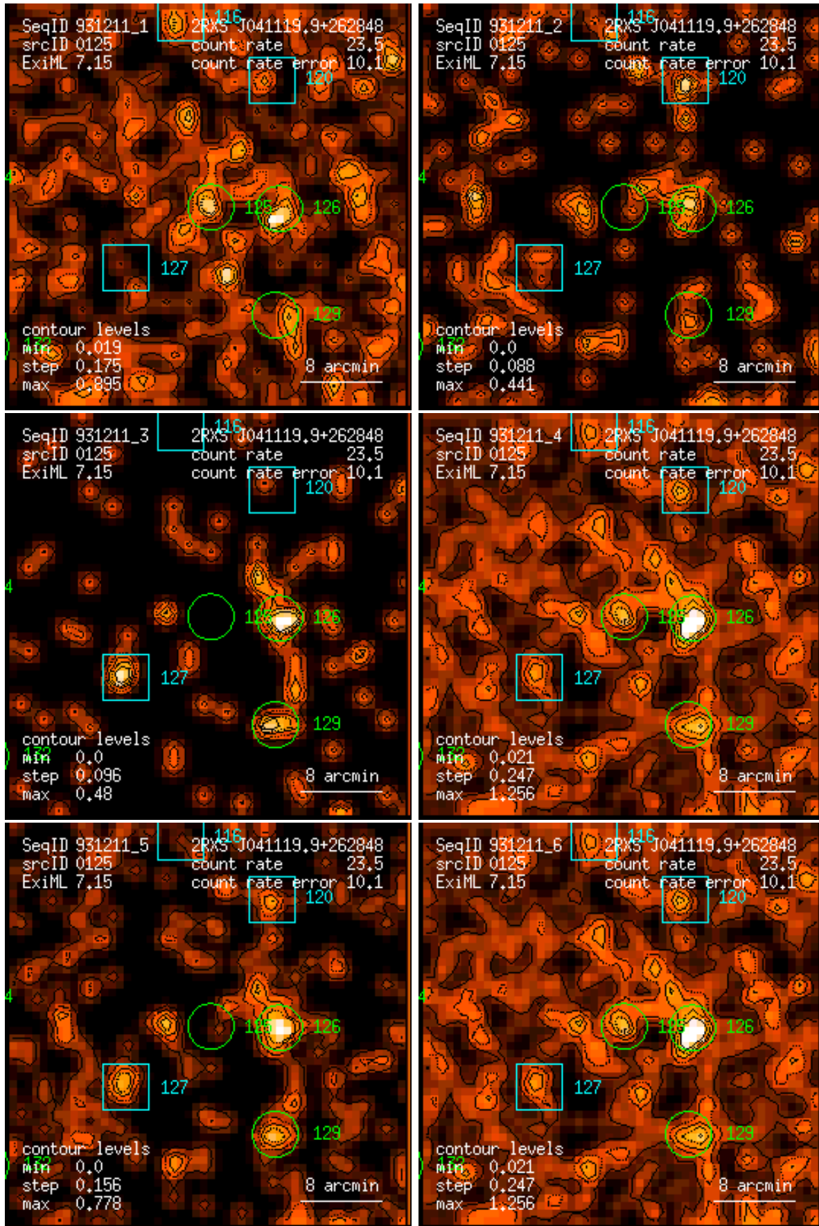
Figure 125: RASS 931211: detection 0125: band rate images, Gaussian filter: (1) PSPC channels 11 – 41, (2) 52 – 90, (3) 91 – 201, (4) 11 – 235, (5) 52 – 201, (6) 11 – 201. Broad band rates in counts/ks. Band rate contour levels in counts/ks/arcmin 2 .
