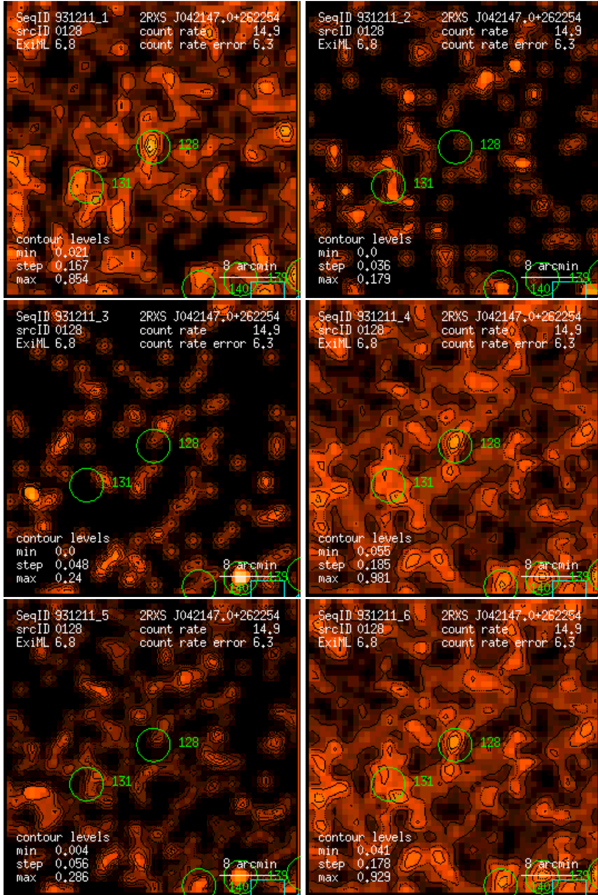
Figure 128: RASS 931211: detection 0128: band rate images, Gaussian filter: (1) PSPC channels 11 – 41, (2) 52 – 90, (3) 91 – 201, (4) 11 – 235, (5) 52 – 201, (6) 11 – 201. Broad band rates in counts/ks. Band rate contour levels in counts/ks/arcmin 2 .
