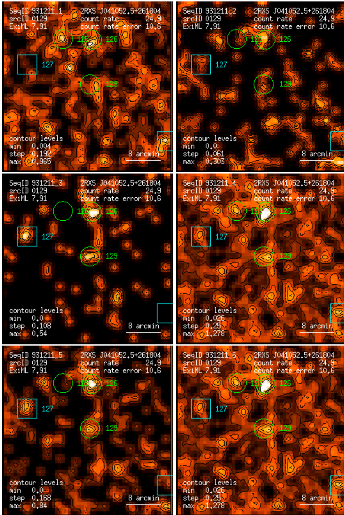
Figure 129: RASS 931211: detection 0129: band rate images, Gaussian filter: (1) PSPC channels 11 – 41, (2) 52 – 90, (3) 91 – 201, (4) 11 – 235, (5) 52 – 201, (6) 11 – 201. Broad band rates in counts/ks. Band rate contour levels in counts/ks/arcmin 2 .
