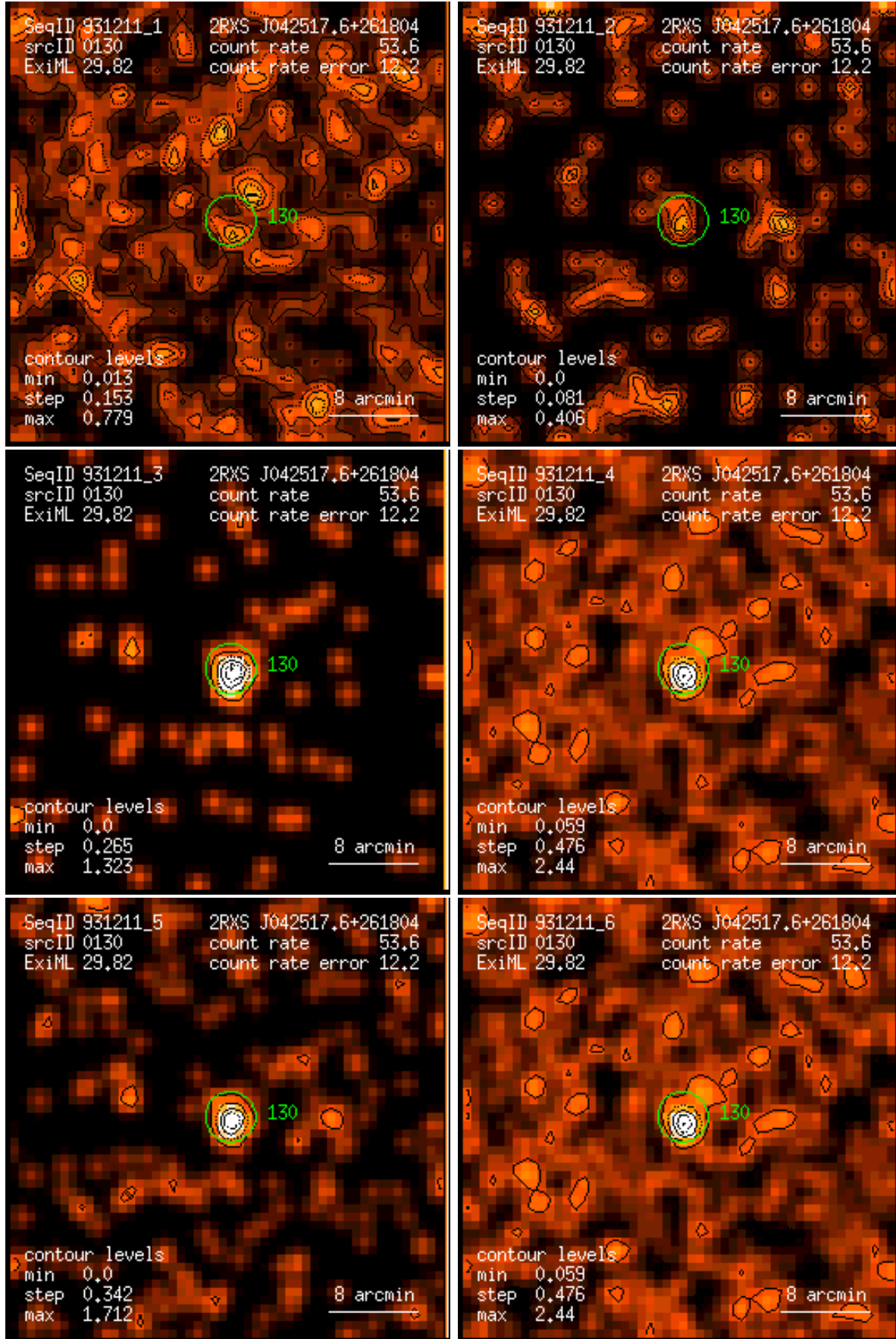
Figure 130: RASS 931211: detection 0130: band rate images, Gaussian filter: (1) PSPC channels 11 – 41, (2) 52 – 90, (3) 91 – 201, (4) 11 – 235, (5) 52 – 201, (6) 11 – 201. Broad band rates in counts/ks. Band rate contour levels in counts/ks/arcmin 2 .
