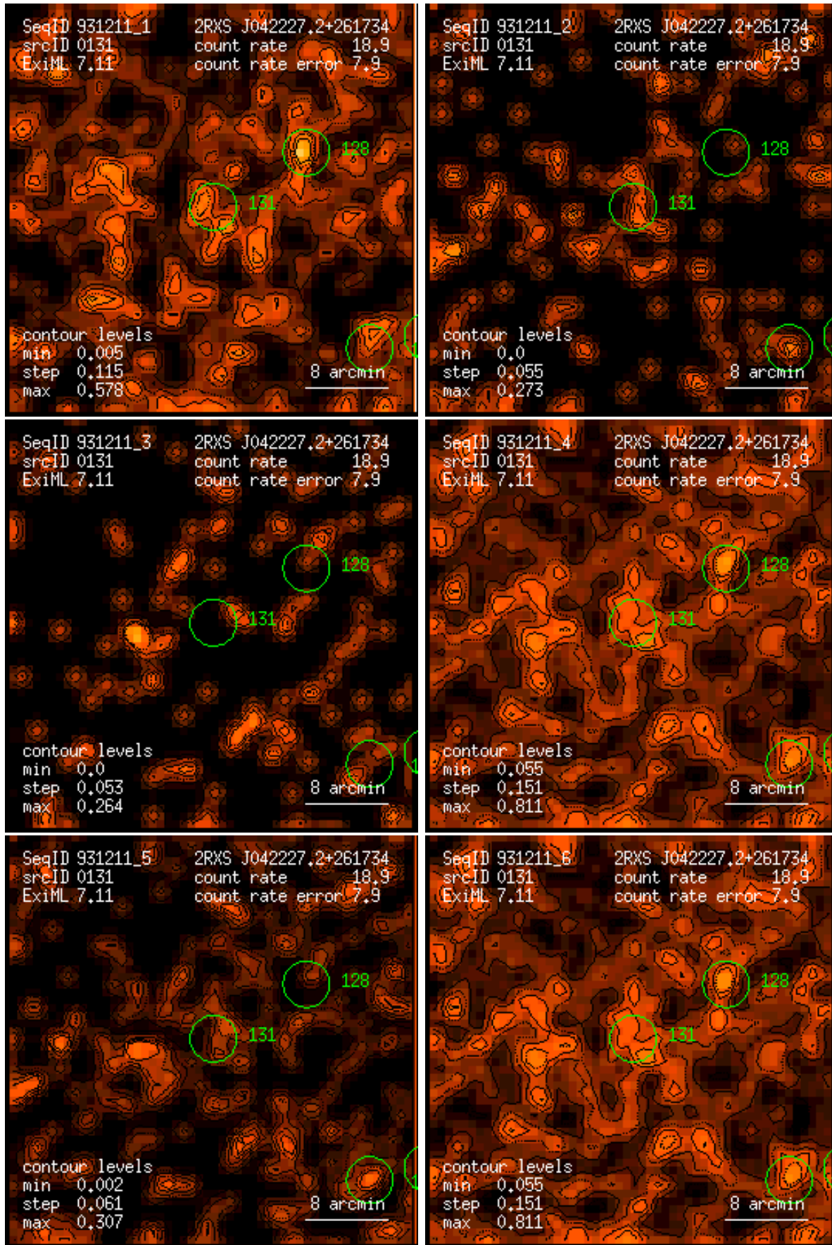
Figure 131: RASS 931211: detection 0131: band rate images, Gaussian filter: (1) PSPC channels 11 – 41, (2) 52 – 90, (3) 91 – 201, (4) 11 – 235, (5) 52 – 201, (6) 11 – 201. Broad band rates in counts/ks. Band rate contour levels in counts/ks/arcmin 2 .
