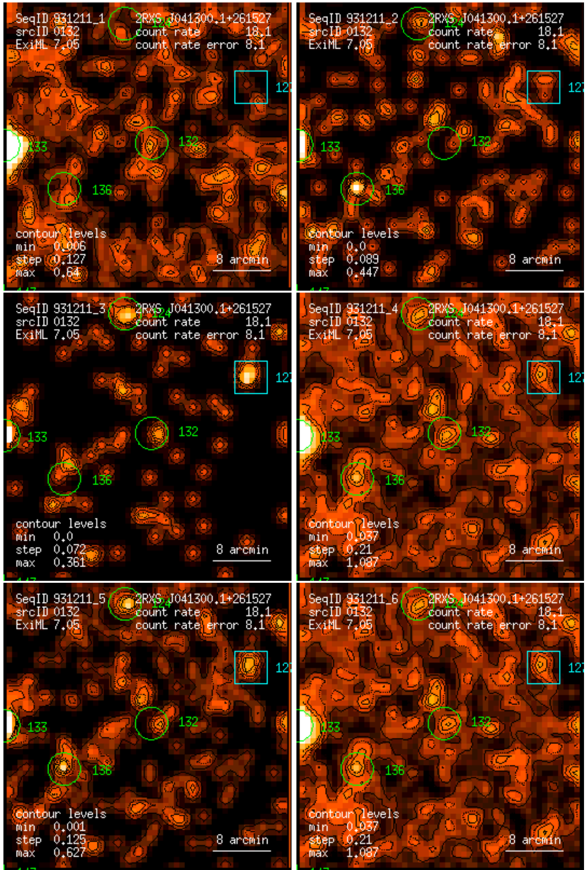
Figure 132: RASS 931211: detection 0132: band rate images, Gaussian filter: (1) PSPC channels 11 – 41, (2) 52 – 90, (3) 91 – 201, (4) 11 – 235, (5) 52 – 201, (6) 11 – 201. Broad band rates in counts/ks. Band rate contour levels in counts/ks/arcmin 2 .
