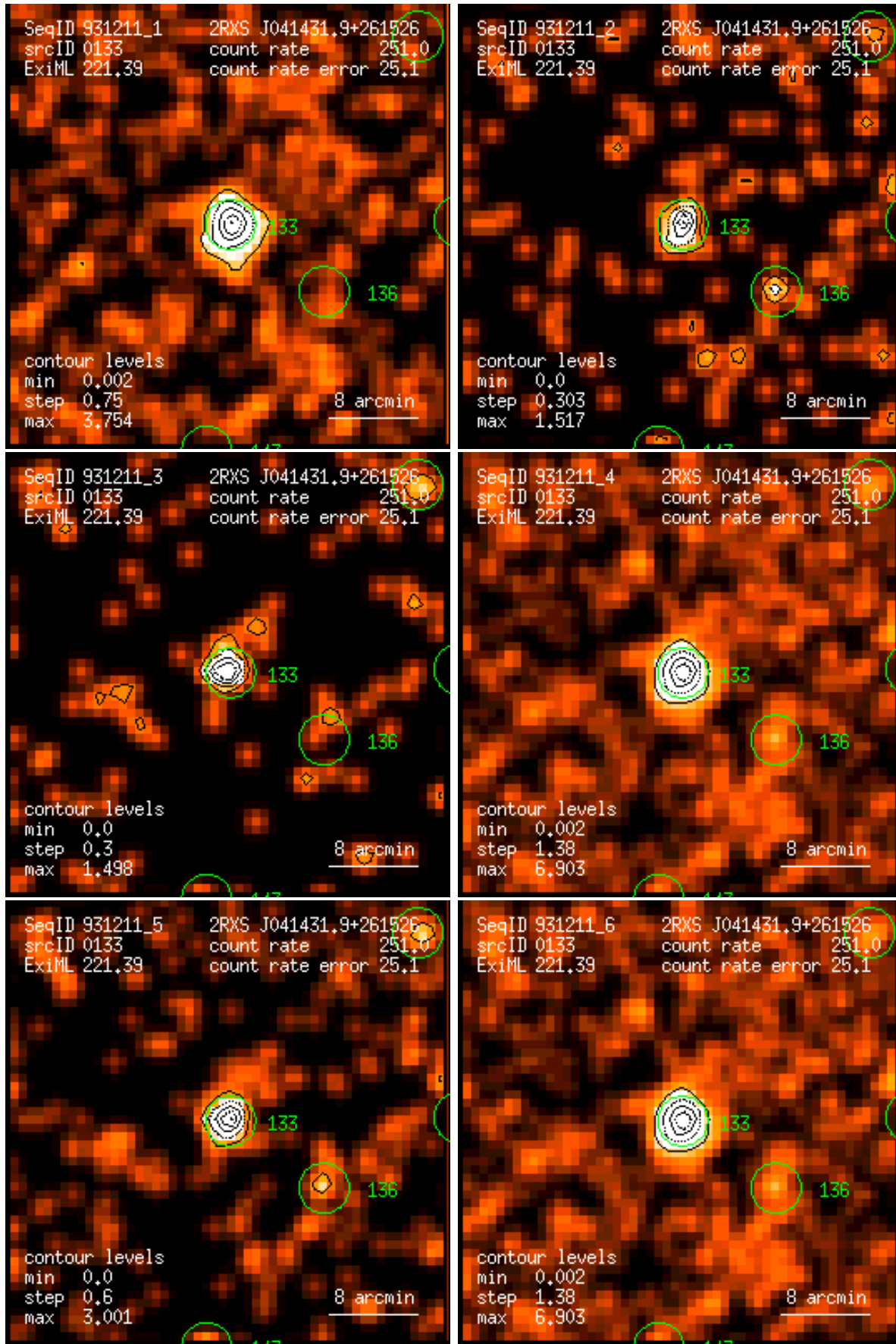
Figure 133: RASS 931211: detection 0133: band rate images, Gaussian filter: (1) PSPC channels 11 – 41, (2) 52 – 90, (3) 91 – 201, (4) 11 – 235, (5) 52 – 201, (6) 11 – 201. Broad band rates in counts/ks. Band rate contour levels in counts/ks/arcmin 2 .
