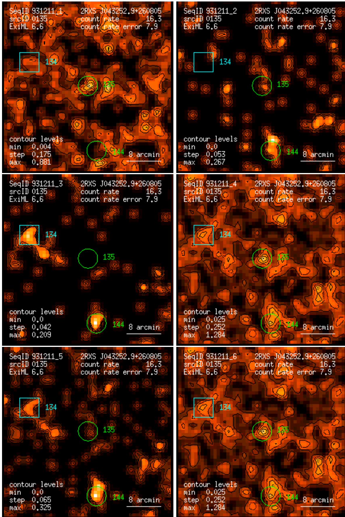
Figure 135: RASS 931211: detection 0135: band rate images, Gaussian filter: (1) PSPC channels 11 – 41, (2) 52 – 90, (3) 91 – 201, (4) 11 – 235, (5) 52 – 201, (6) 11 – 201. Broad band rates in counts/ks. Band rate contour levels in counts/ks/arcmin 2 .
