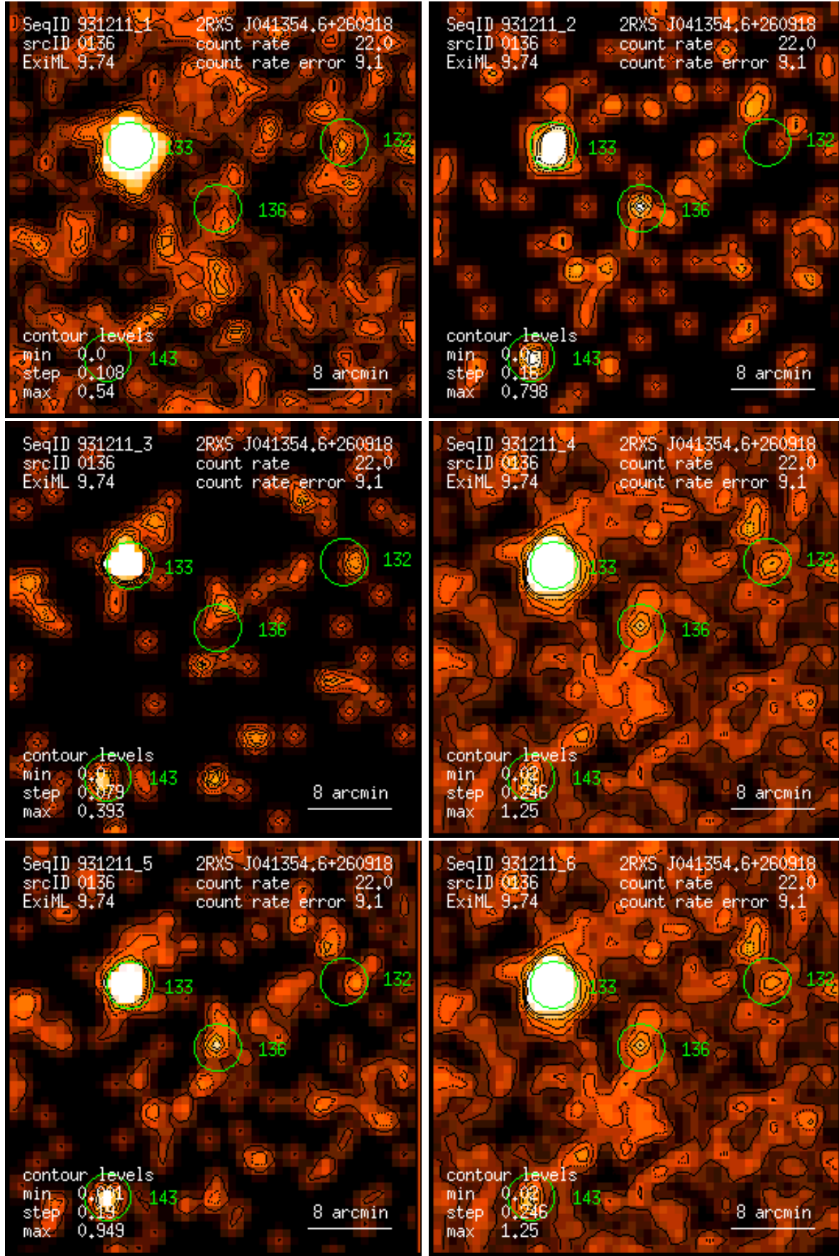
Figure 136: RASS 931211: detection 0136: band rate images, Gaussian filter: (1) PSPC channels 11 – 41, (2) 52 – 90, (3) 91 – 201, (4) 11 – 235, (5) 52 – 201, (6) 11 – 201. Broad band rates in counts/ks. Band rate contour levels in counts/ks/arcmin 2 .
