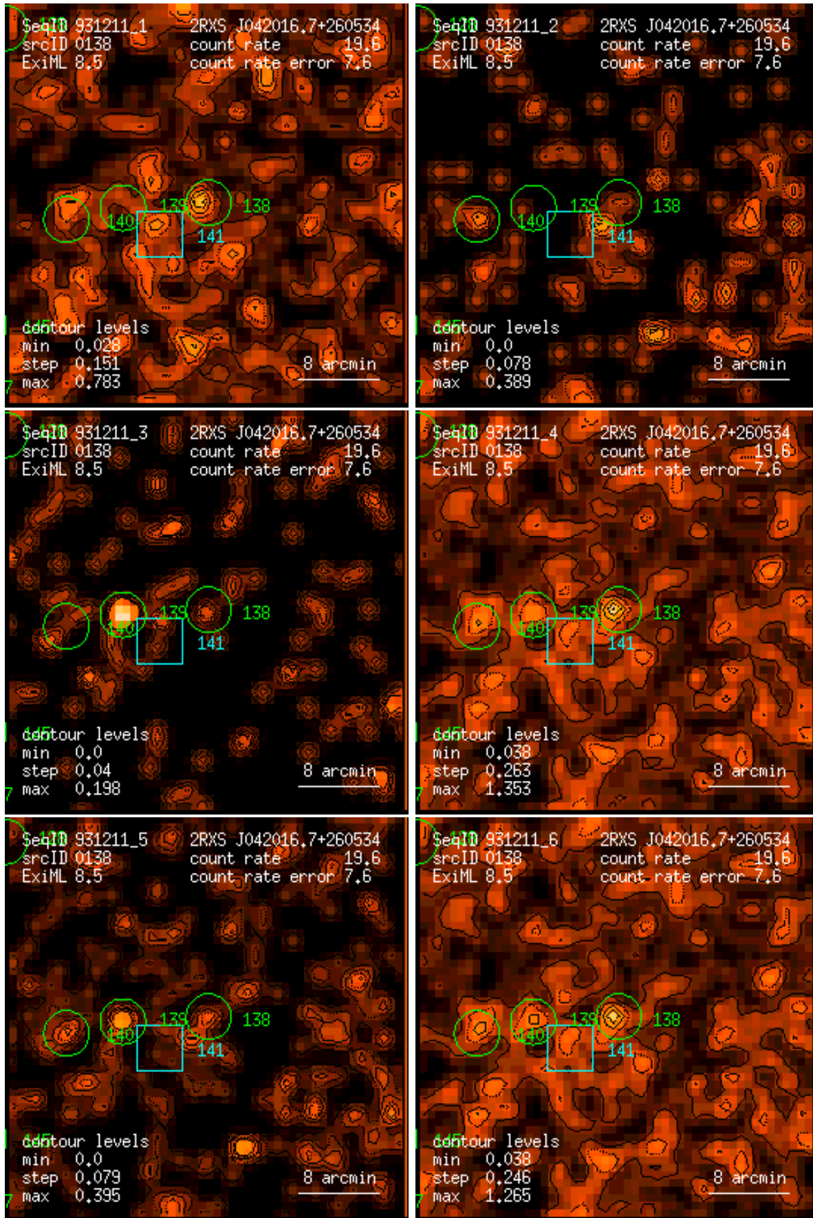
Figure 138: RASS 931211: detection 0138: band rate images, Gaussian filter: (1) PSPC channels 11 – 41, (2) 52 – 90, (3) 91 – 201, (4) 11 – 235, (5) 52 – 201, (6) 11 – 201. Broad band rates in counts/ks. Band rate contour levels in counts/ks/arcmin 2 .
