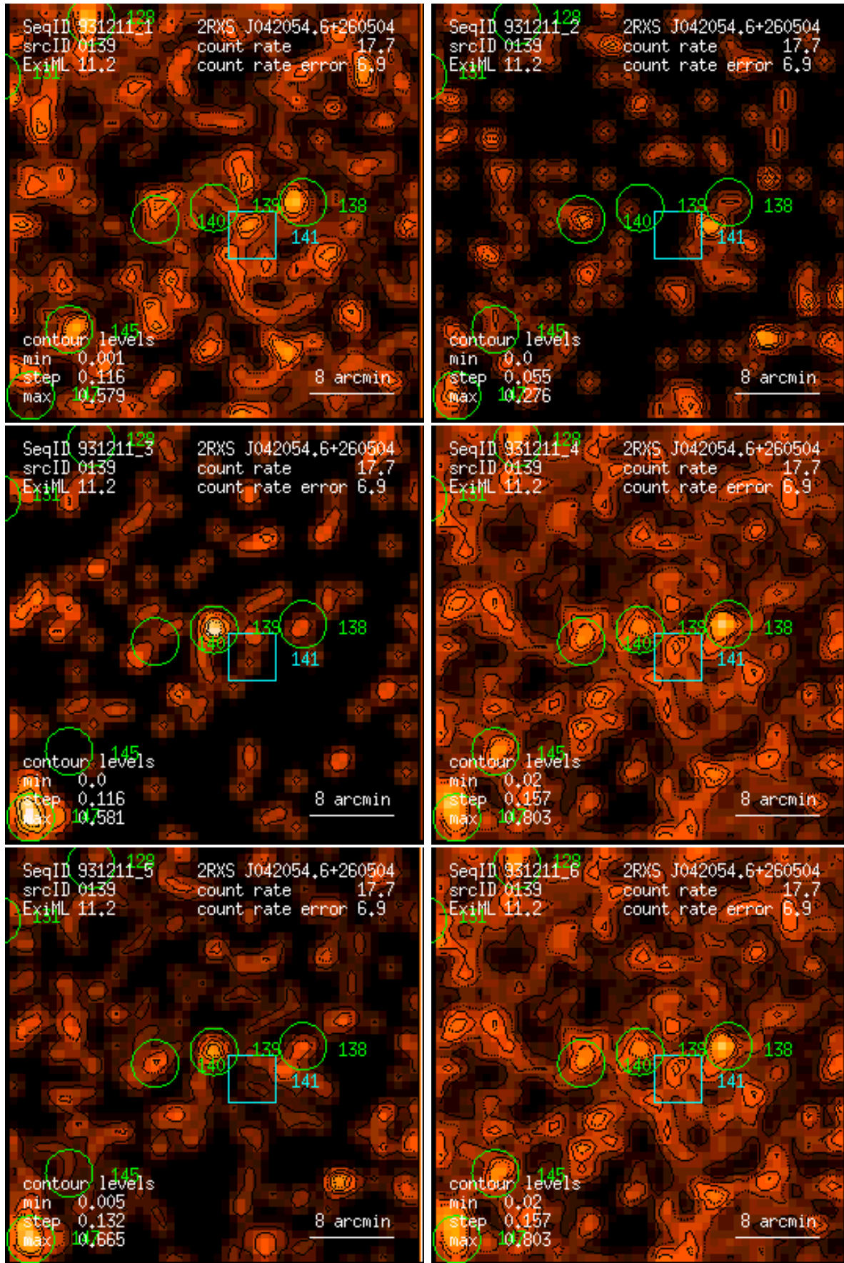
Figure 139: RASS 931211: detection 0139: band rate images, Gaussian filter: (1) PSPC channels 11 – 41, (2) 52 – 90, (3) 91 – 201, (4) 11 – 235, (5) 52 – 201, (6) 11 – 201. Broad band rates in counts/ks. Band rate contour levels in counts/ks/arcmin 2 .
