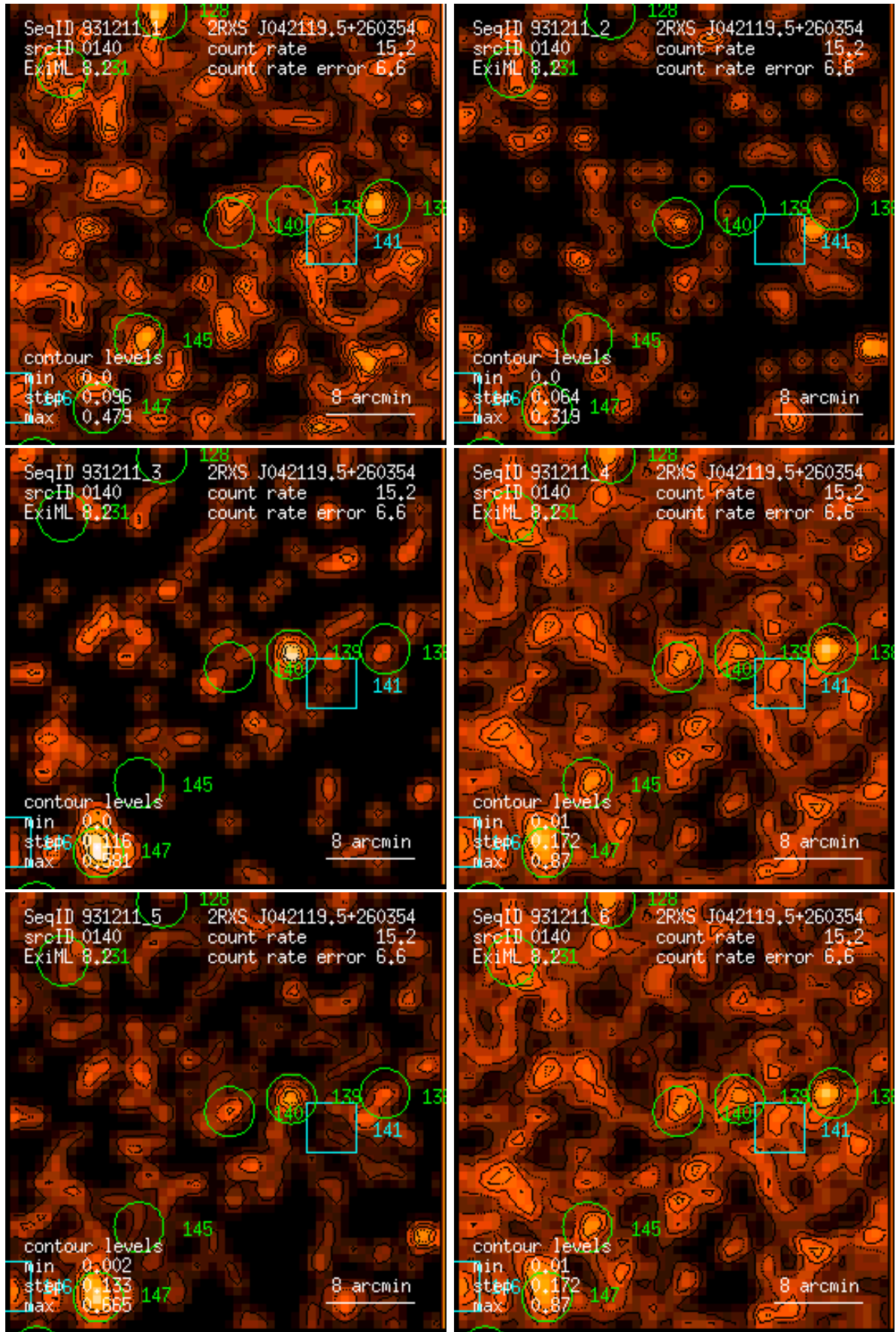
Figure 140: RASS 931211: detection 0140: band rate images, Gaussian filter: (1) PSPC channels 11 – 41, (2) 52 – 90, (3) 91 – 201, (4) 11 – 235, (5) 52 – 201, (6) 11 – 201. Broad band rates in counts/ks. Band rate contour levels in counts/ks/arcmin 2 .
