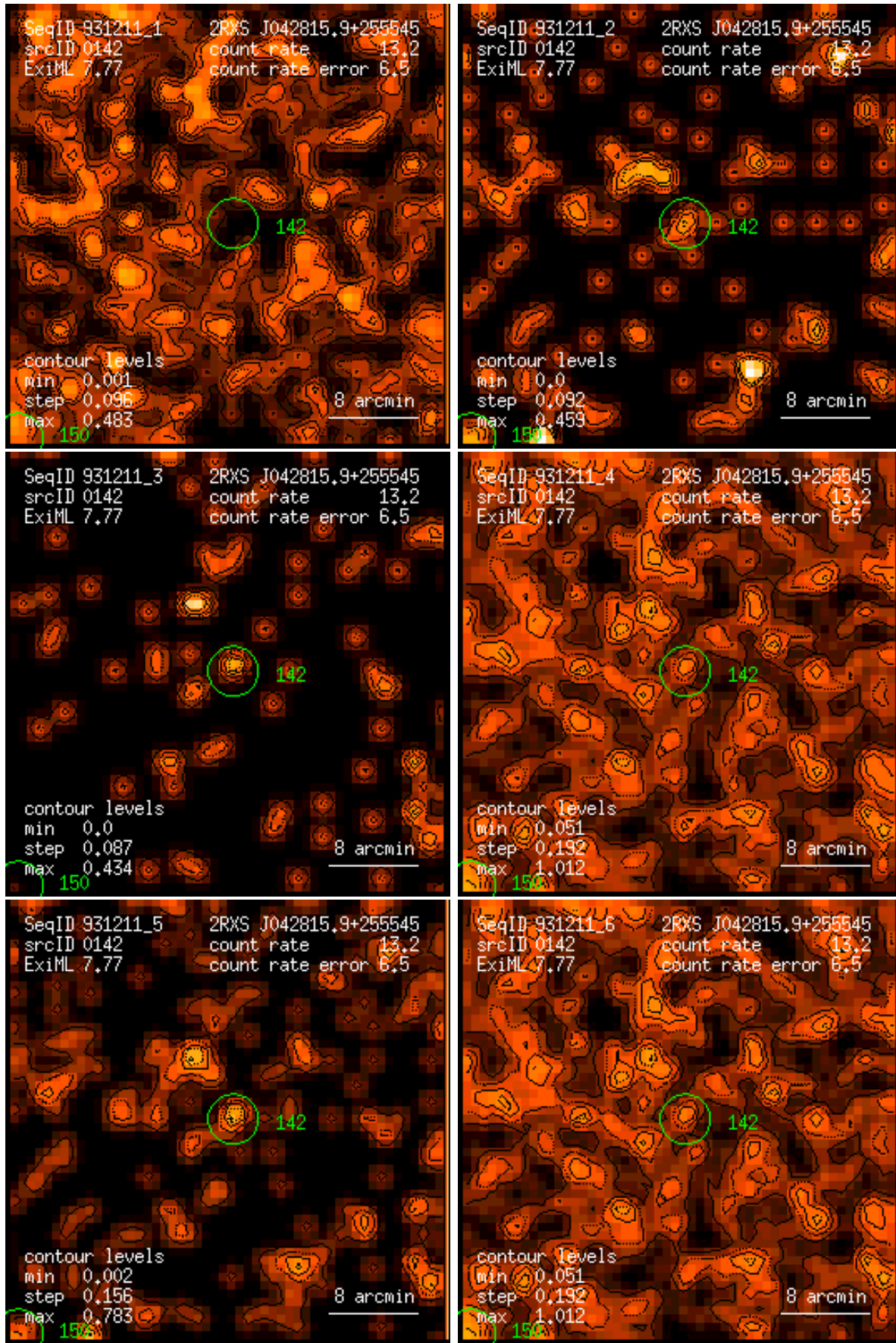
Figure 142: RASS 931211: detection 0142: band rate images, Gaussian filter: (1) PSPC channels 11 – 41, (2) 52 – 90, (3) 91 – 201, (4) 11 – 235, (5) 52 – 201, (6) 11 – 201. Broad band rates in counts/ks. Band rate contour levels in counts/ks/arcmin 2 .
