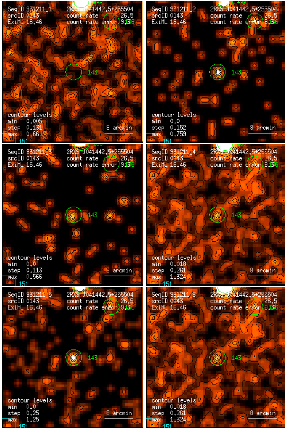
Figure 143: RASS 931211: detection 0143: band rate images, Gaussian filter: (1) PSPC channels 11 – 41, (2) 52 – 90, (3) 91 – 201, (4) 11 – 235, (5) 52 – 201, (6) 11 – 201. Broad band rates in counts/ks. Band rate contour levels in counts/ks/arcmin 2 .
