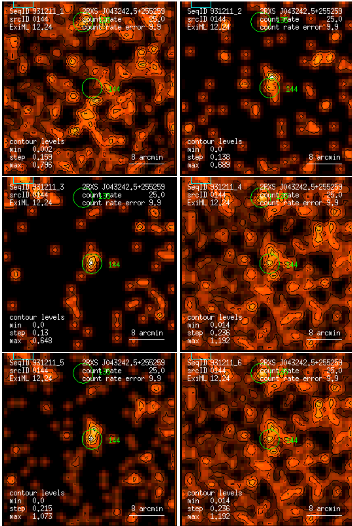
Figure 144: RASS 931211: detection 0144: band rate images, Gaussian filter: (1) PSPC channels 11 – 41, (2) 52 – 90, (3) 91 – 201, (4) 11 – 235, (5) 52 – 201, (6) 11 – 201. Broad band rates in counts/ks. Band rate contour levels in counts/ks/arcmin 2 .
