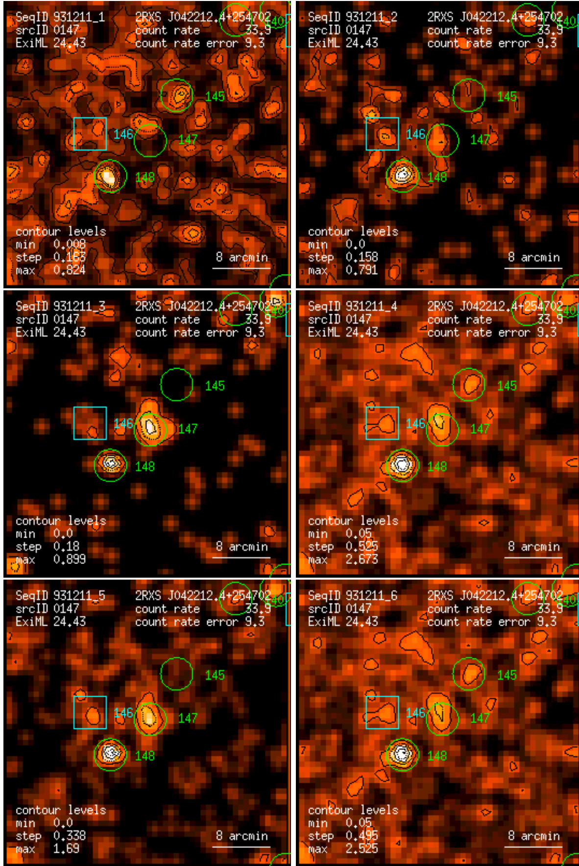
Figure 147: RASS 931211: detection 0147: band rate images, Gaussian filter: (1) PSPC channels 11 – 41, (2) 52 – 90, (3) 91 – 201, (4) 11 – 235, (5) 52 – 201, (6) 11 – 201. Broad band rates in counts/ks. Band rate contour levels in counts/ks/arcmin 2 .
