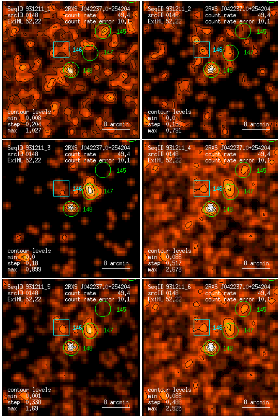
Figure 148: RASS 931211: detection 0148: band rate images, Gaussian filter: (1) PSPC channels 11 – 41, (2) 52 – 90, (3) 91 – 201, (4) 11 – 235, (5) 52 – 201, (6) 11 – 201. Broad band rates in counts/ks. Band rate contour levels in counts/ks/arcmin 2 .
