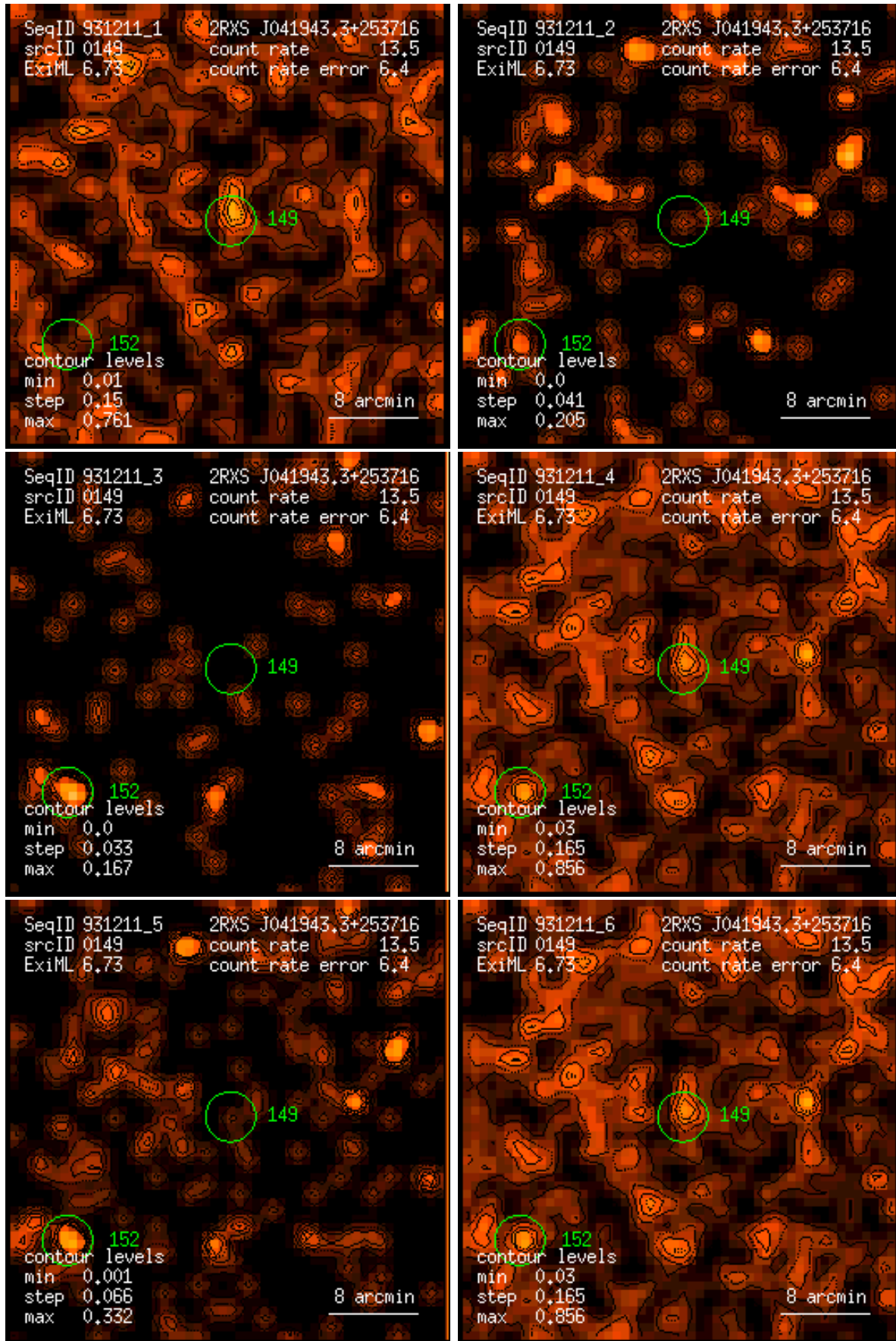
Figure 149: RASS 931211: detection 0149: band rate images, Gaussian filter: (1) PSPC channels 11 – 41, (2) 52 – 90, (3) 91 – 201, (4) 11 – 235, (5) 52 – 201, (6) 11 – 201. Broad band rates in counts/ks. Band rate contour levels in counts/ks/arcmin 2 .
