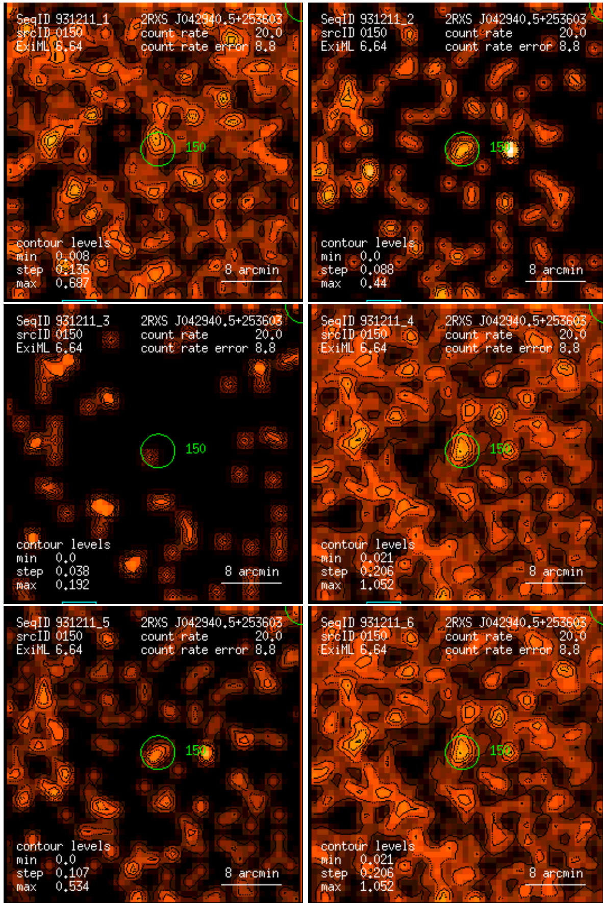
Figure 150: RASS 931211: detection 0150: band rate images, Gaussian filter: (1) PSPC channels 11 – 41, (2) 52 – 90, (3) 91 – 201, (4) 11 – 235, (5) 52 – 201, (6) 11 – 201. Broad band rates in counts/ks. Band rate contour levels in counts/ks/arcmin 2 .
