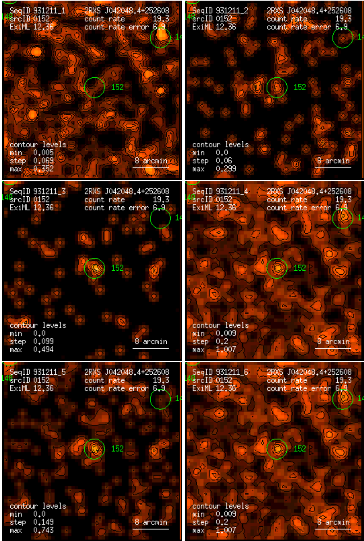
Figure 152: RASS 931211: detection 0152: band rate images, Gaussian filter: (1) PSPC channels 11 – 41, (2) 52 – 90, (3) 91 – 201, (4) 11 – 235, (5) 52 – 201, (6) 11 – 201. Broad band rates in counts/ks. Band rate contour levels in counts/ks/arcmin 2 .
