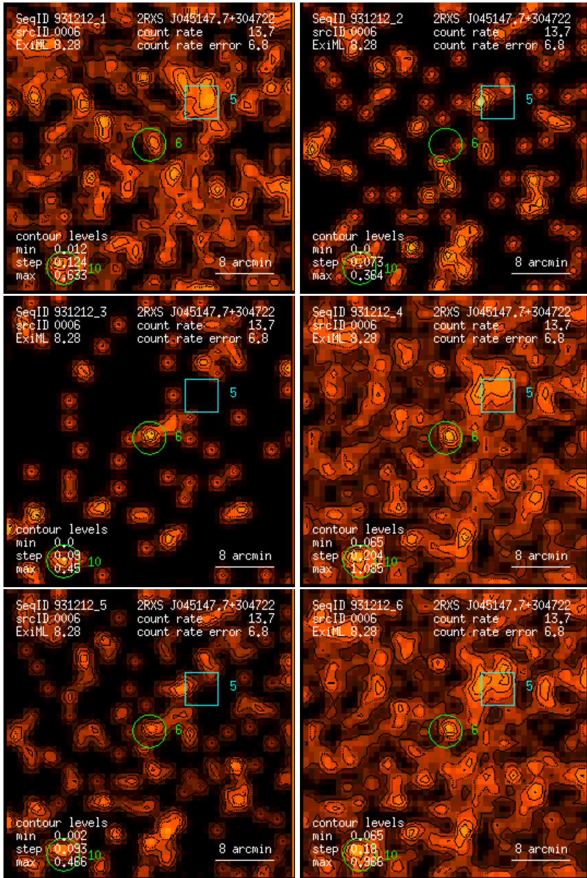
Figure 6: RASS 931212: detection 0006: band rate images, Gaussian filter: (1) PSPC channels 11 – 41, (2) 52 – 90, (3) 91 – 201, (4) 11 – 235, (5) 52 – 201, (6) 11 – 201. Broad band rates in counts/ks. Band rate contour levels in counts/ks/arcmin 2 .
