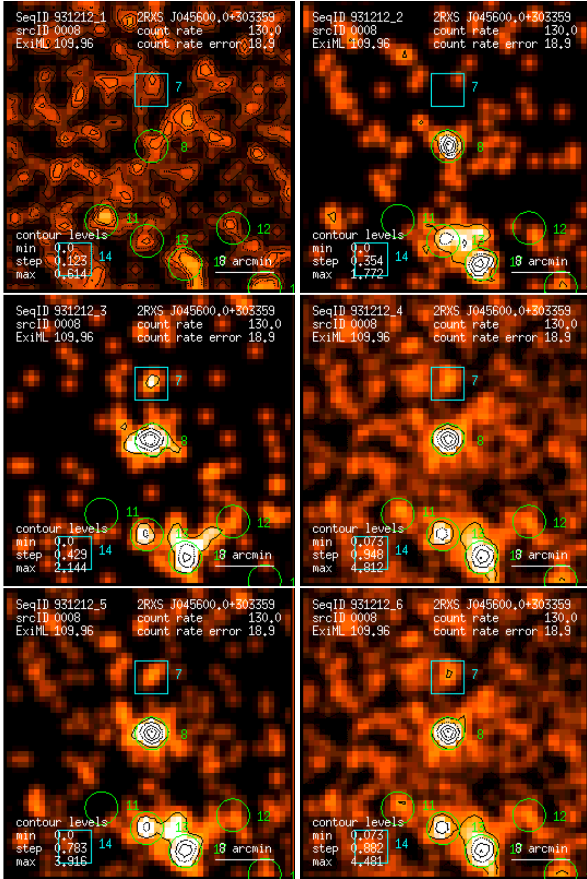
Figure 8: RASS 931212: detection 0008: band rate images, Gaussian filter: (1) PSPC channels 11 – 41, (2) 52 – 90, (3) 91 – 201, (4) 11 – 235, (5) 52 – 201, (6) 11 – 201. Broad band rates in counts/ks. Band rate contour levels in counts/ks/arcmin 2 .
