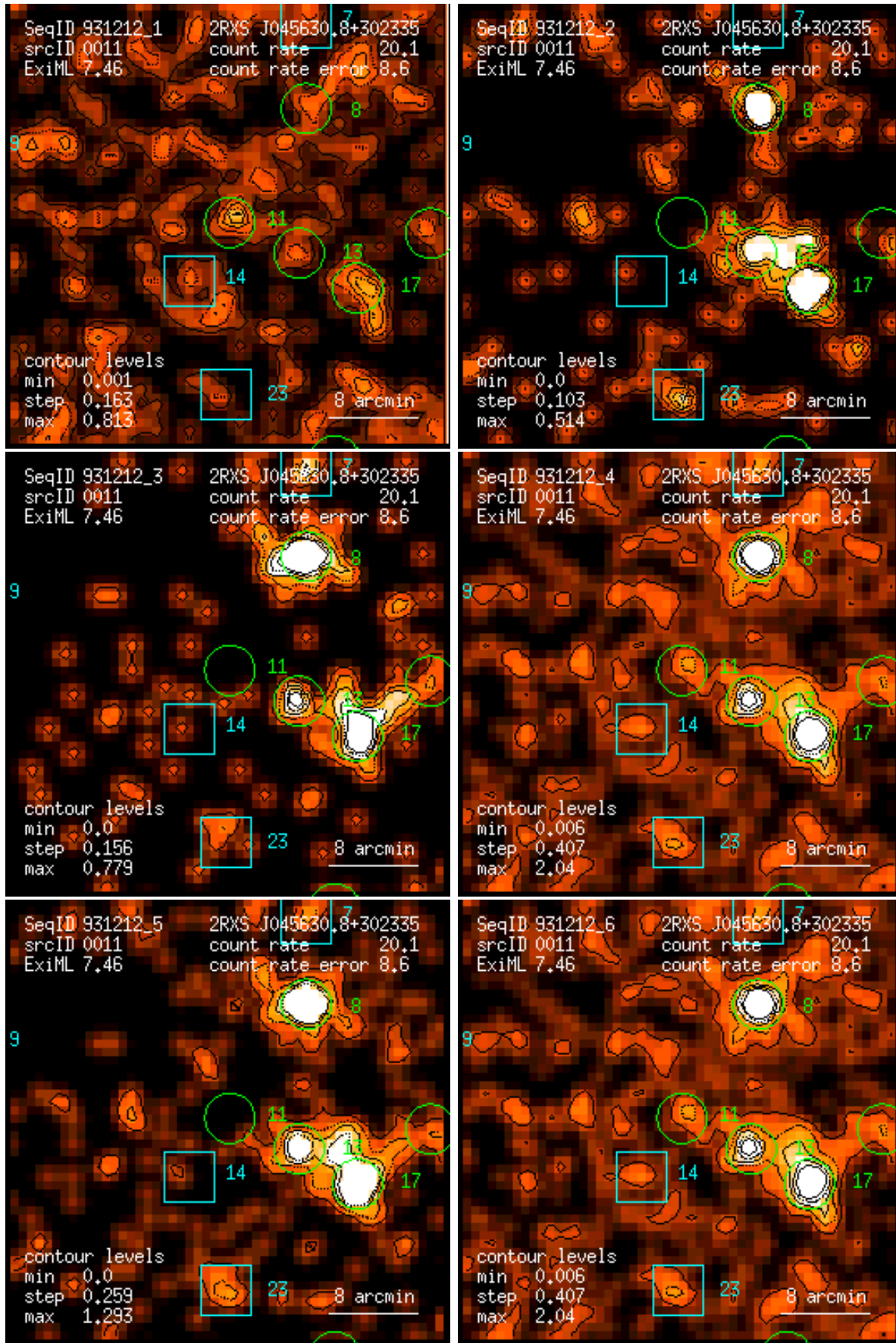
Figure 11: RASS 931212: detection 0011: band rate images, Gaussian filter: (1) PSPC channels 11 – 41, (2) 52 – 90, (3) 91 – 201, (4) 11 – 235, (5) 52 – 201, (6) 11 – 201. Broad band rates in counts/ks. Band rate contour levels in counts/ks/arcmin 2 .
