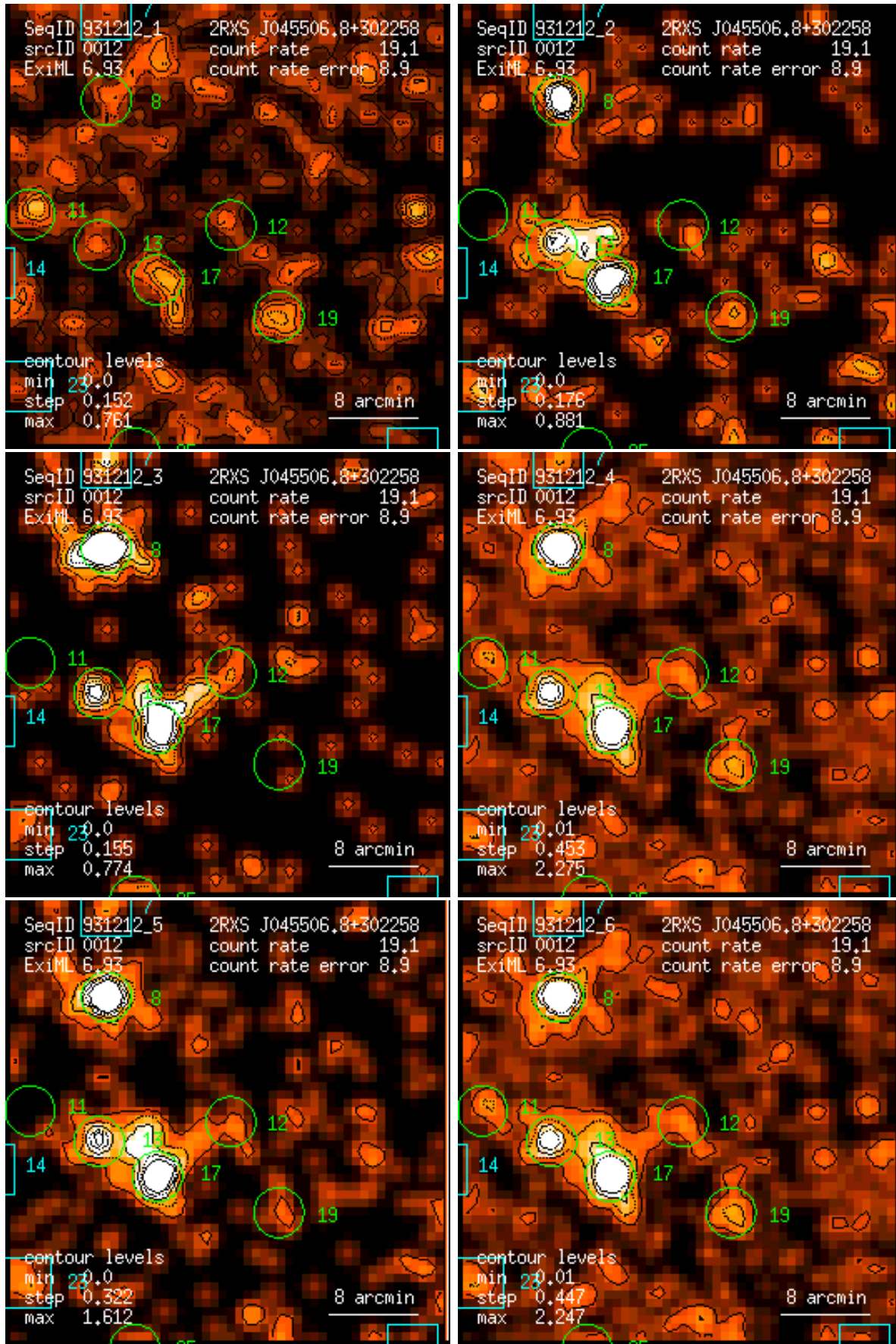
Figure 12: RASS 931212: detection 0012: band rate images, Gaussian filter: (1) PSPC channels 11 – 41, (2) 52 – 90, (3) 91 – 201, (4) 11 – 235, (5) 52 – 201, (6) 11 – 201. Broad band rates in counts/ks. Band rate contour levels in counts/ks/arcmin 2 .
