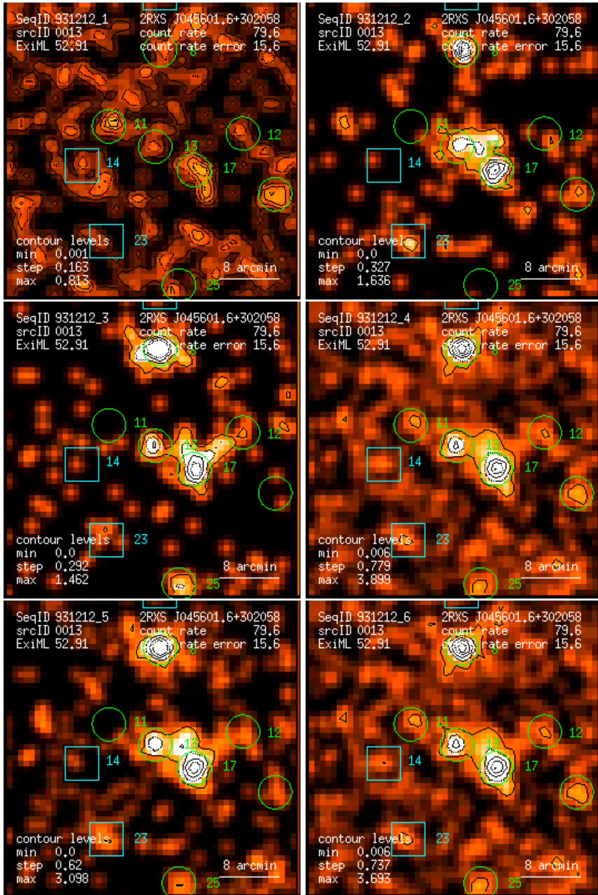
Figure 13: RASS 931212: detection 0013: band rate images, Gaussian filter: (1) PSPC channels 11 – 41, (2) 52 – 90, (3) 91 – 201, (4) 11 – 235, (5) 52 – 201, (6) 11 – 201. Broad band rates in counts/ks. Band rate contour levels in counts/ks/arcmin 2 .
