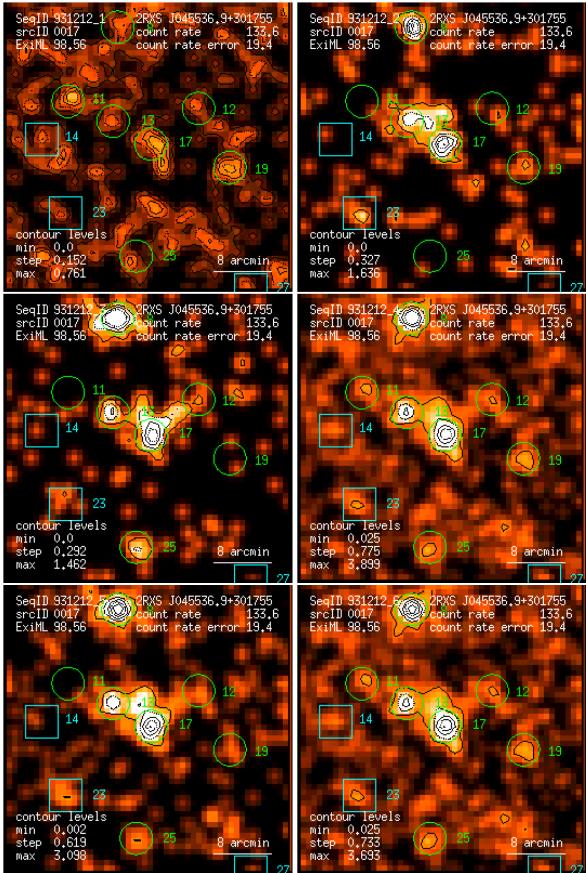
Figure 17: RASS 931212: detection 0017: band rate images, Gaussian filter: (1) PSPC channels 11 – 41, (2) 52 – 90, (3) 91 – 201, (4) 11 – 235, (5) 52 – 201, (6) 11 – 201. Broad band rates in counts/ks. Band rate contour levels in counts/ks/arcmin 2 .
