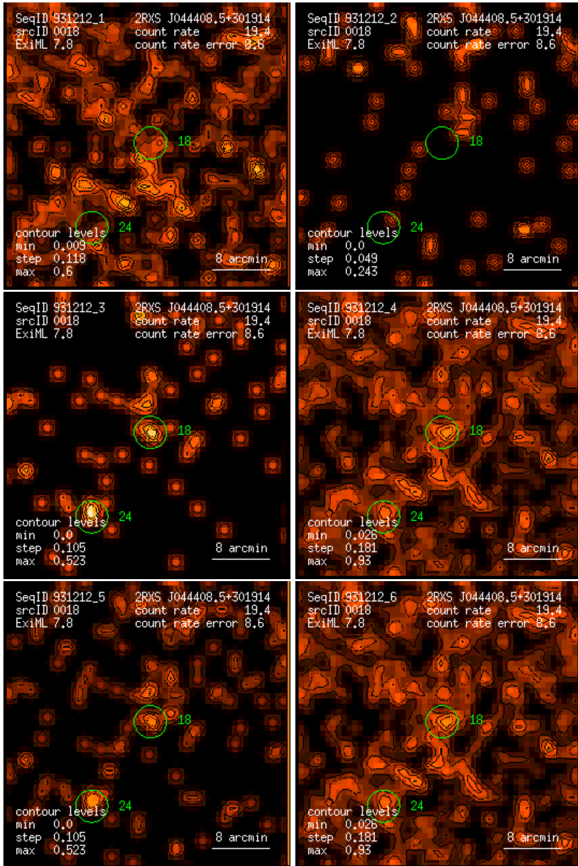
Figure 18: RASS 931212: detection 0018: band rate images, Gaussian filter: (1) PSPC channels 11 – 41, (2) 52 – 90, (3) 91 – 201, (4) 11 – 235, (5) 52 – 201, (6) 11 – 201. Broad band rates in counts/ks. Band rate contour levels in counts/ks/arcmin 2 .
