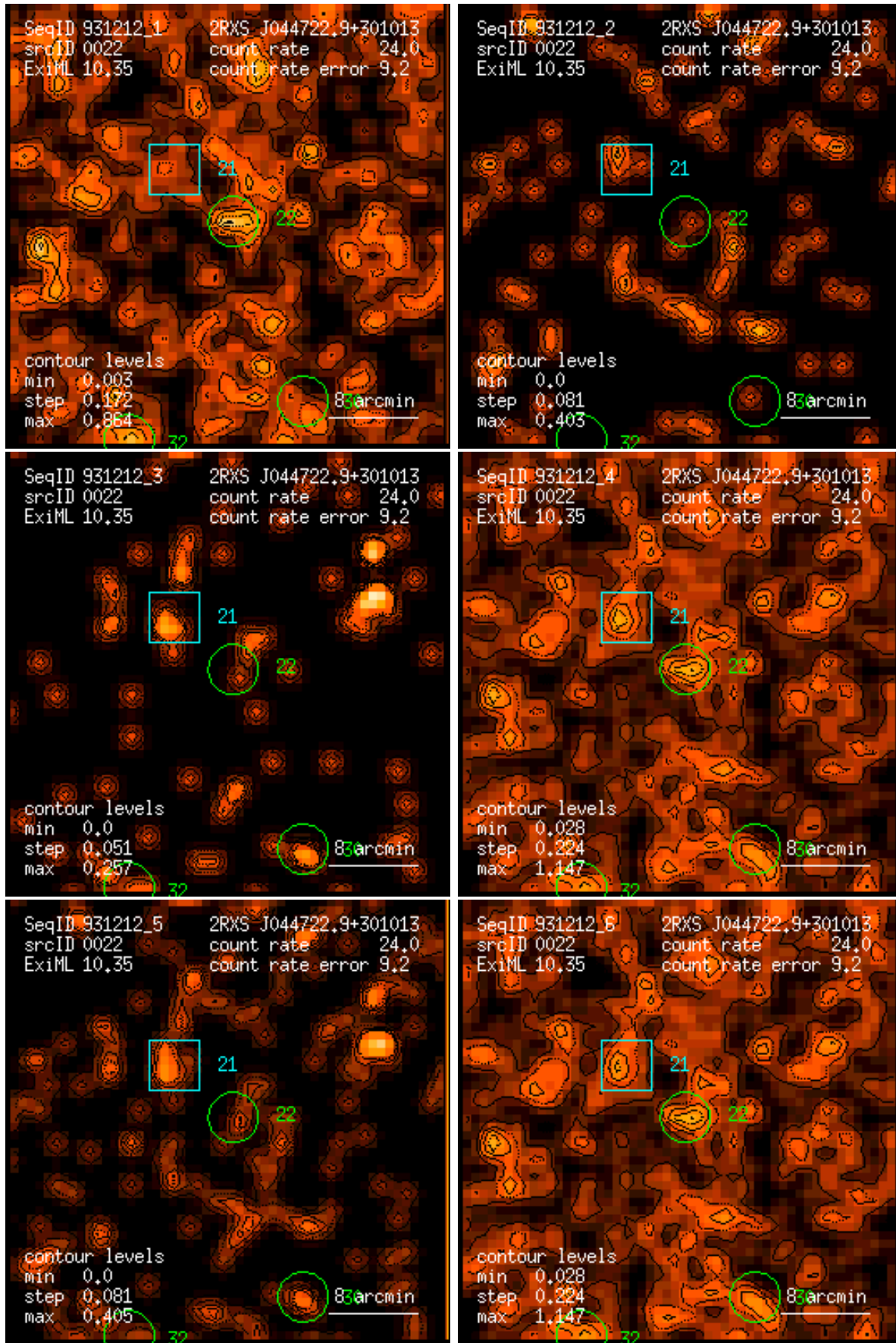
Figure 22: RASS 931212: detection 0022: band rate images, Gaussian filter: (1) PSPC channels 11 – 41, (2) 52 – 90, (3) 91 – 201, (4) 11 – 235, (5) 52 – 201, (6) 11 – 201. Broad band rates in counts/ks. Band rate contour levels in counts/ks/arcmin 2 .
