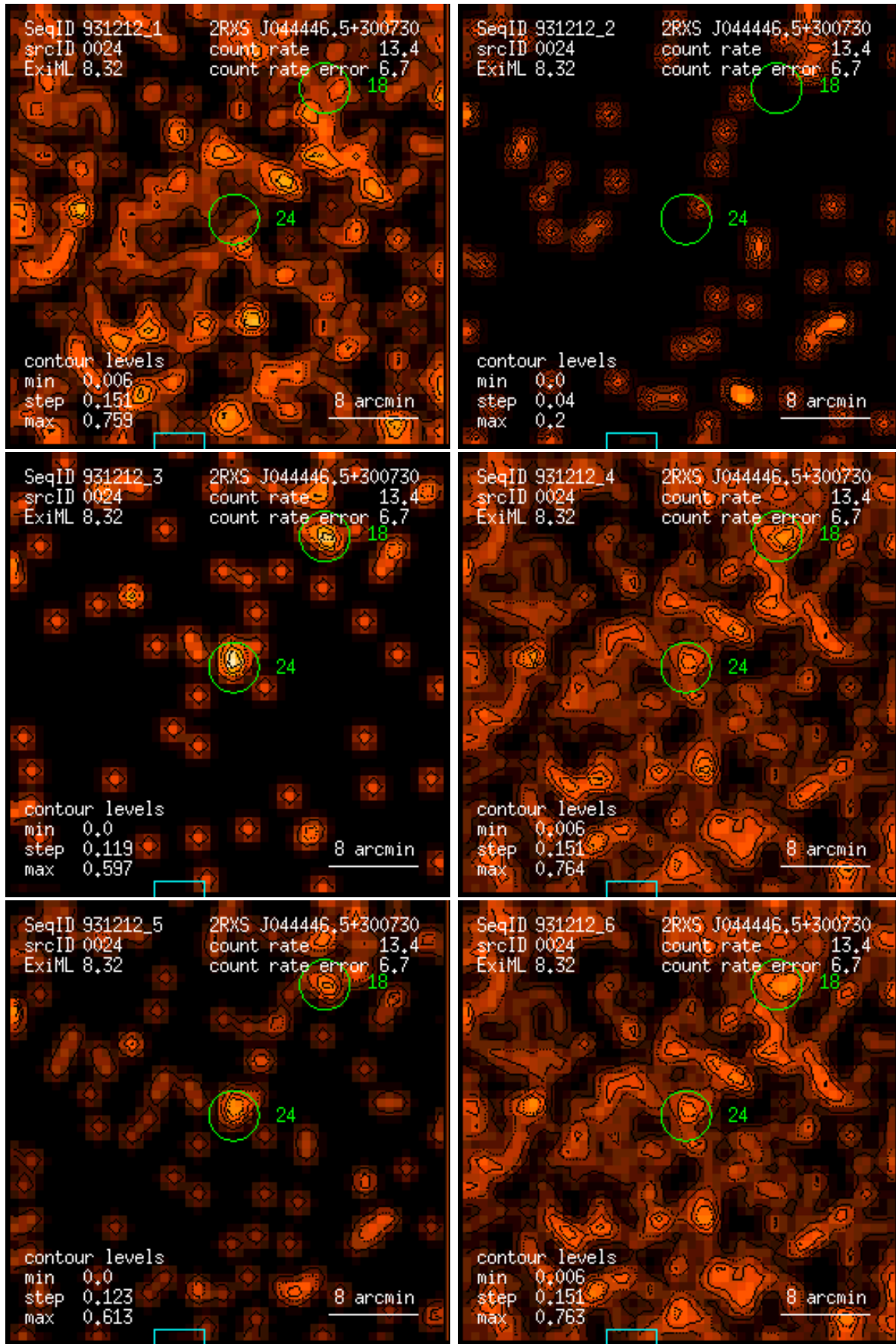
Figure 24: RASS 931212: detection 0024: band rate images, Gaussian filter: (1) PSPC channels 11 – 41, (2) 52 – 90, (3) 91 – 201, (4) 11 – 235, (5) 52 – 201, (6) 11 – 201. Broad band rates in counts/ks. Band rate contour levels in counts/ks/arcmin 2 .
