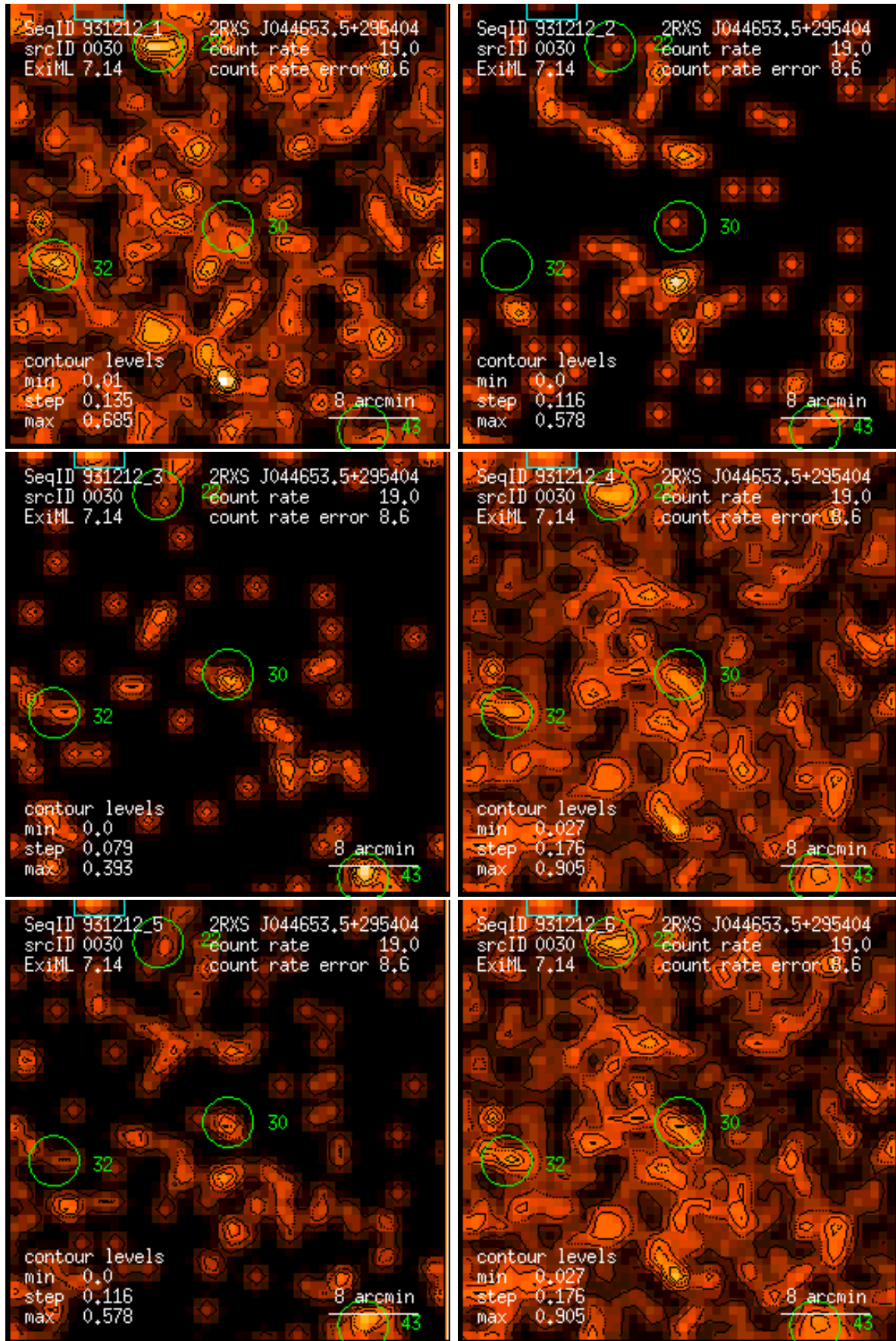
Figure 30: RASS 931212: detection 0030: band rate images, Gaussian filter: (1) PSPC channels 11 – 41, (2) 52 – 90, (3) 91 – 201, (4) 11 – 235, (5) 52 – 201, (6) 11 – 201. Broad band rates in counts/ks. Band rate contour levels in counts/ks/arcmin 2 .
