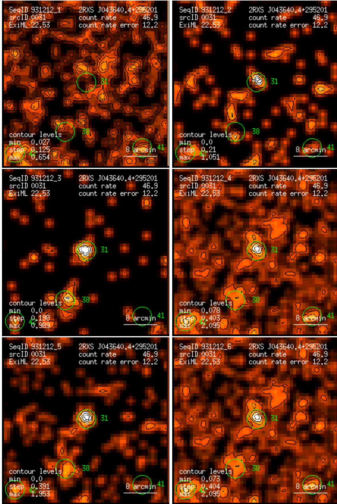
Figure 31: RASS 931212: detection 0031: band rate images, Gaussian filter: (1) PSPC channels 11 – 41, (2) 52 – 90, (3) 91 – 201, (4) 11 – 235, (5) 52 – 201, (6) 11 – 201. Broad band rates in counts/ks. Band rate contour levels in counts/ks/arcmin 2 .
