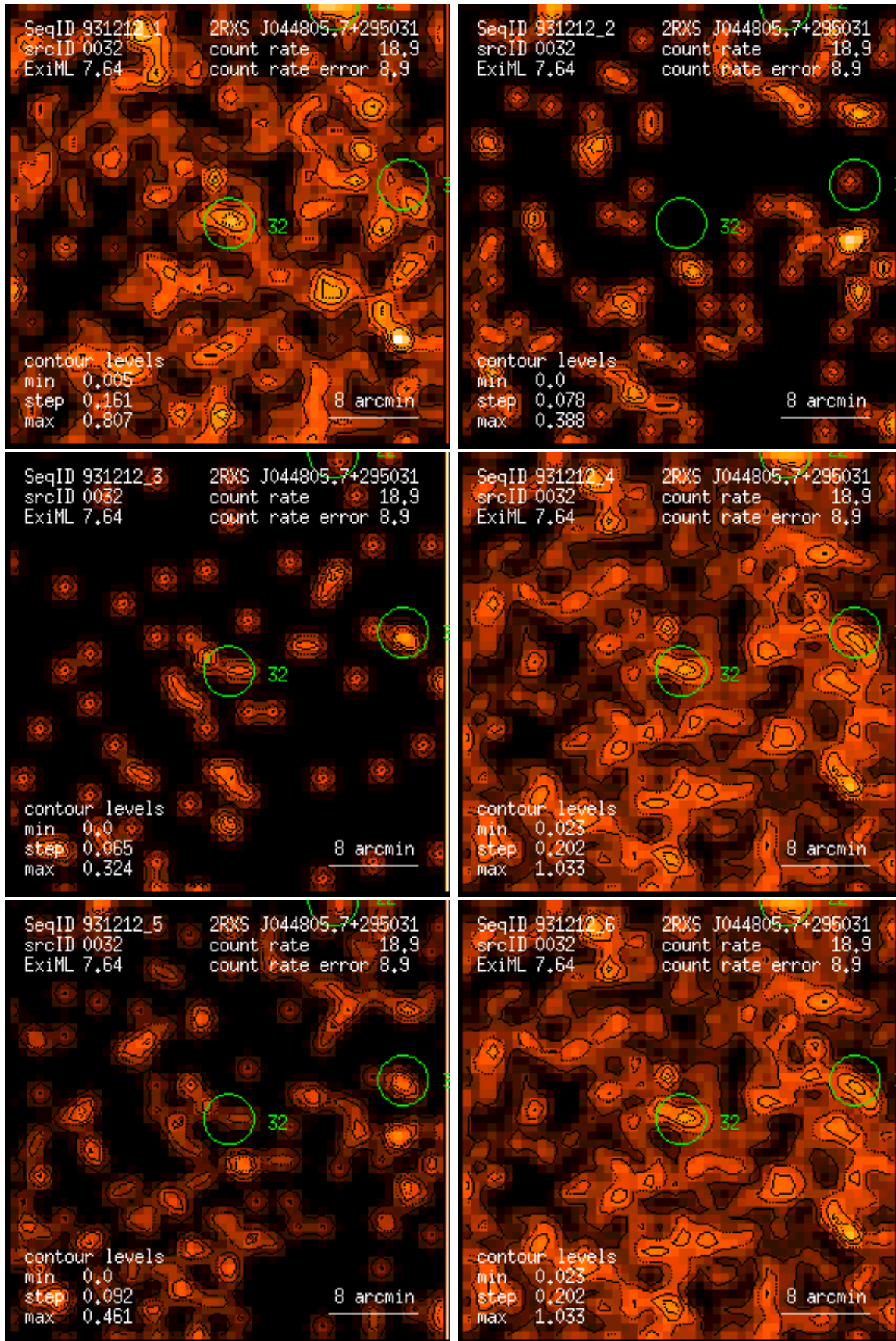
Figure 32: RASS 931212: detection 0032: band rate images, Gaussian filter: (1) PSPC channels 11 – 41, (2) 52 – 90, (3) 91 – 201, (4) 11 – 235, (5) 52 – 201, (6) 11 – 201. Broad band rates in counts/ks. Band rate contour levels in counts/ks/arcmin 2 .
