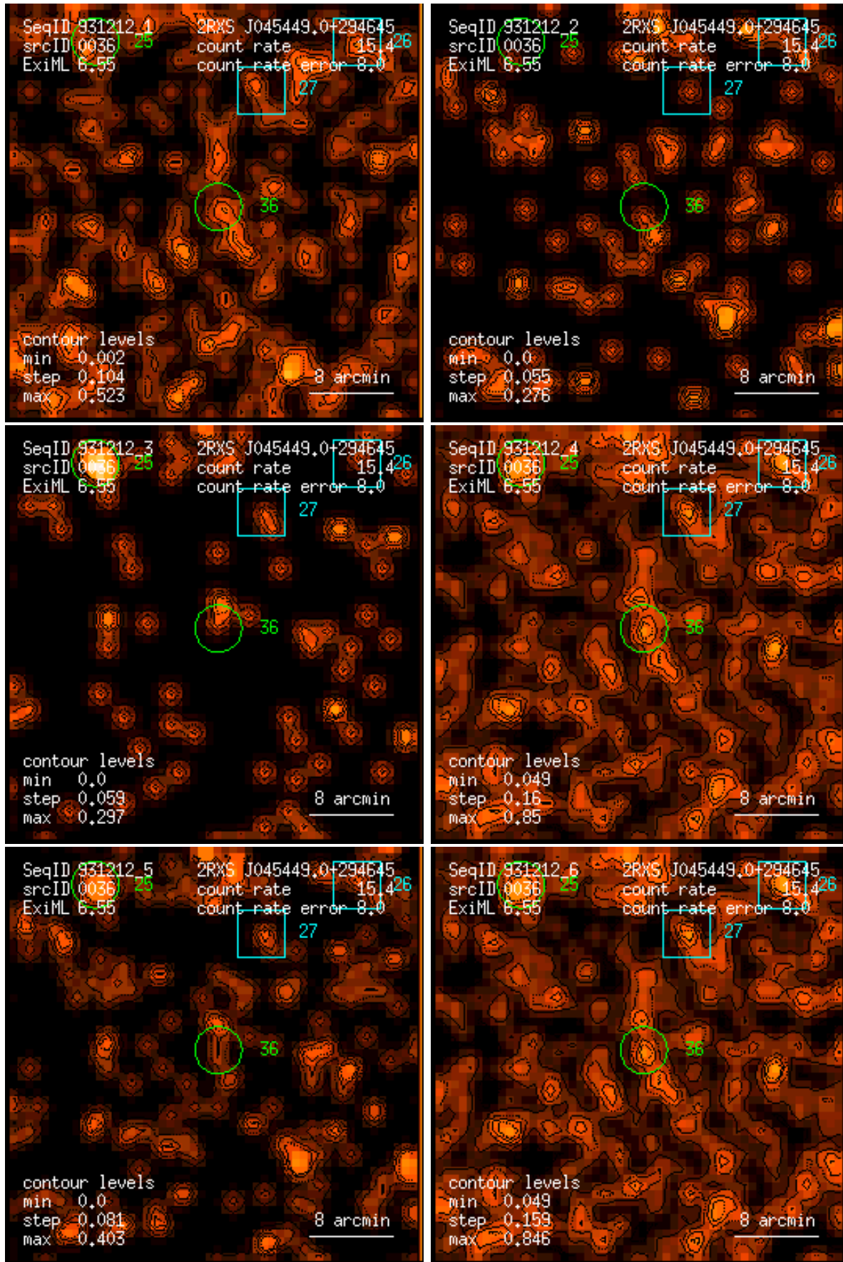
Figure 36: RASS 931212: detection 0036: band rate images, Gaussian filter: (1) PSPC channels 11 – 41, (2) 52 – 90, (3) 91 – 201, (4) 11 – 235, (5) 52 – 201, (6) 11 – 201. Broad band rates in counts/ks. Band rate contour levels in counts/ks/arcmin 2 .
