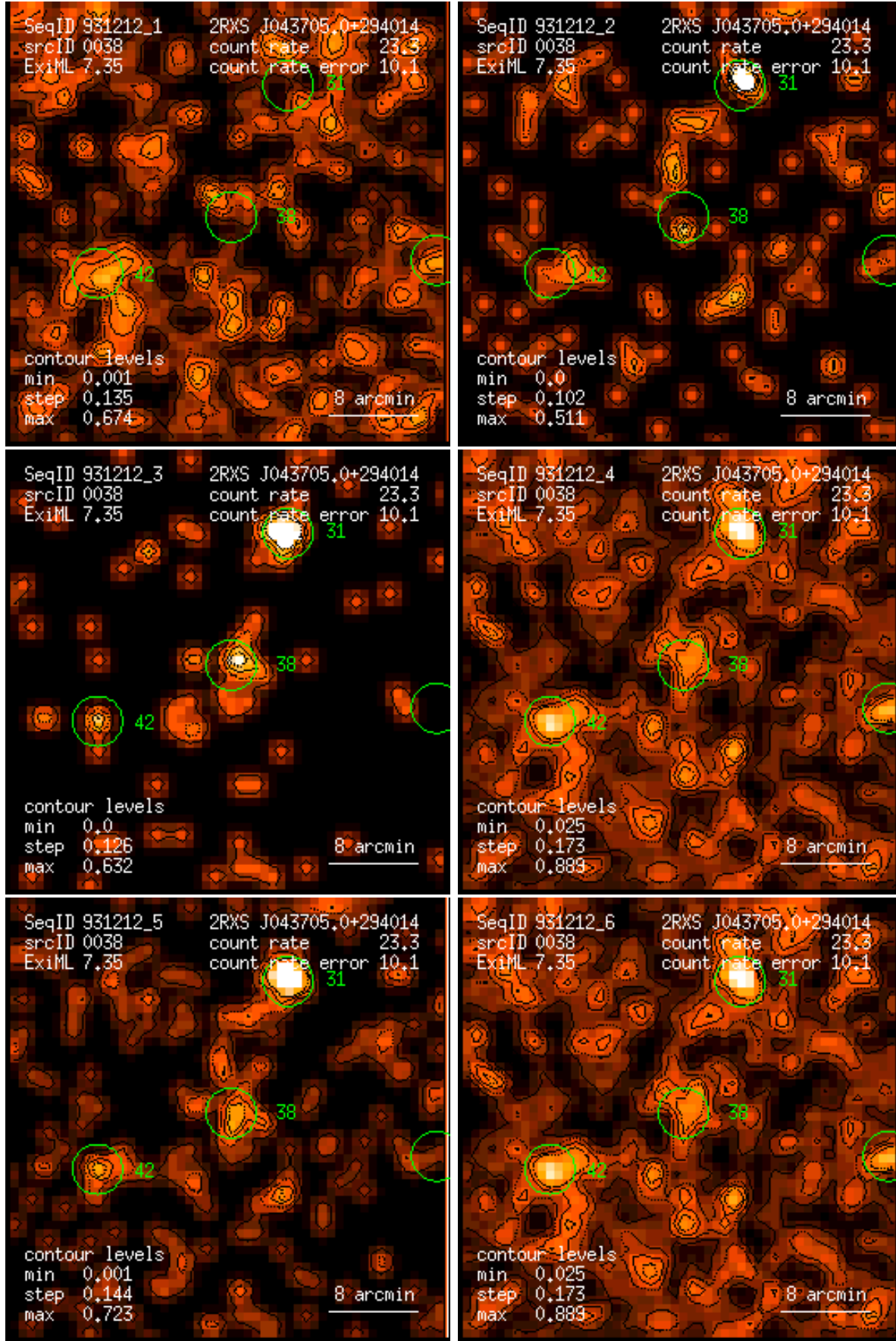
Figure 38: RASS 931212: detection 0038: band rate images, Gaussian filter: (1) PSPC channels 11 – 41, (2) 52 – 90, (3) 91 – 201, (4) 11 – 235, (5) 52 – 201, (6) 11 – 201. Broad band rates in counts/ks. Band rate contour levels in counts/ks/arcmin 2 .
