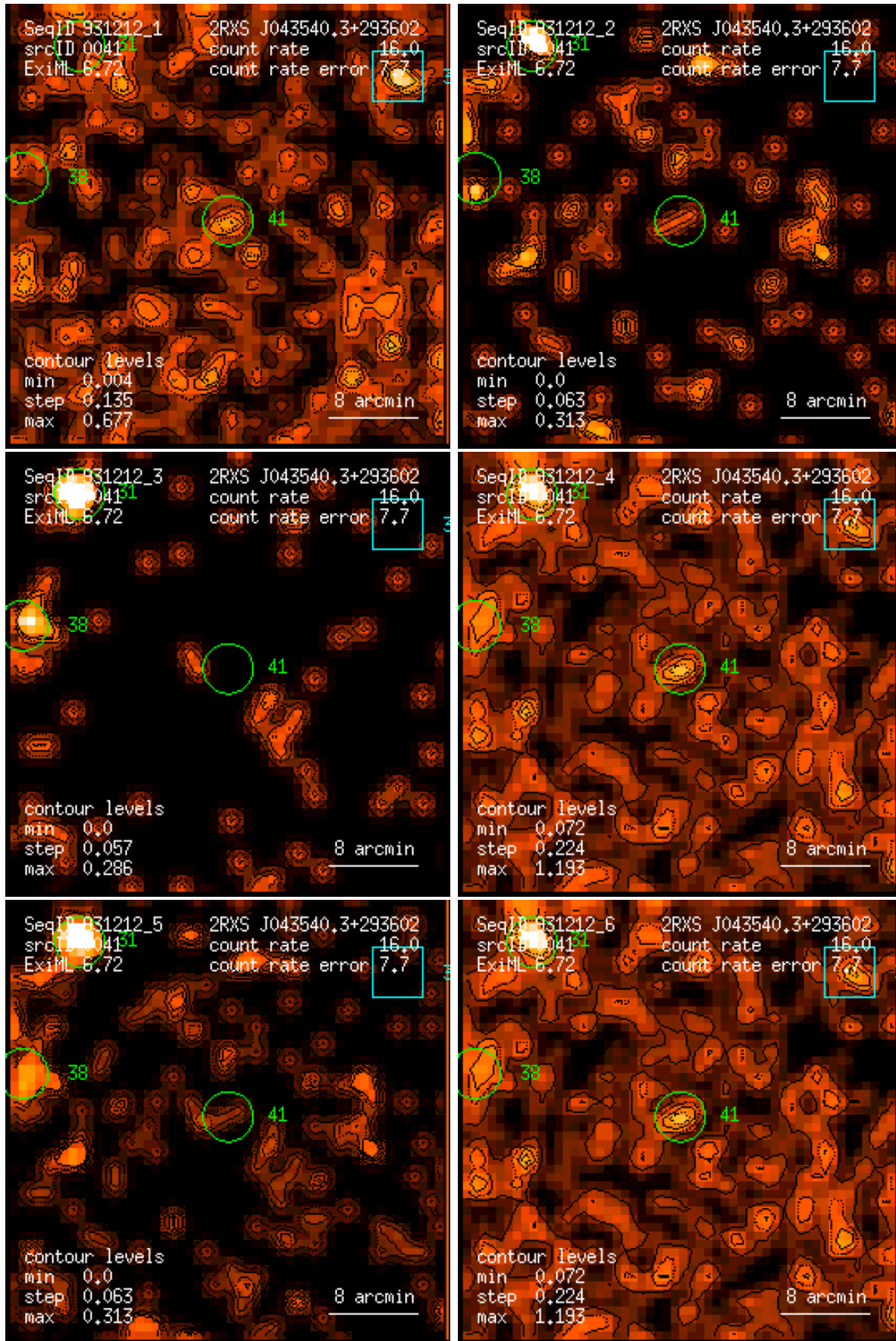
Figure 41: RASS 931212: detection 0041: band rate images, Gaussian filter: (1) PSPC channels 11 – 41, (2) 52 – 90, (3) 91 – 201, (4) 11 – 235, (5) 52 – 201, (6) 11 – 201. Broad band rates in counts/ks. Band rate contour levels in counts/ks/arcmin 2 .
