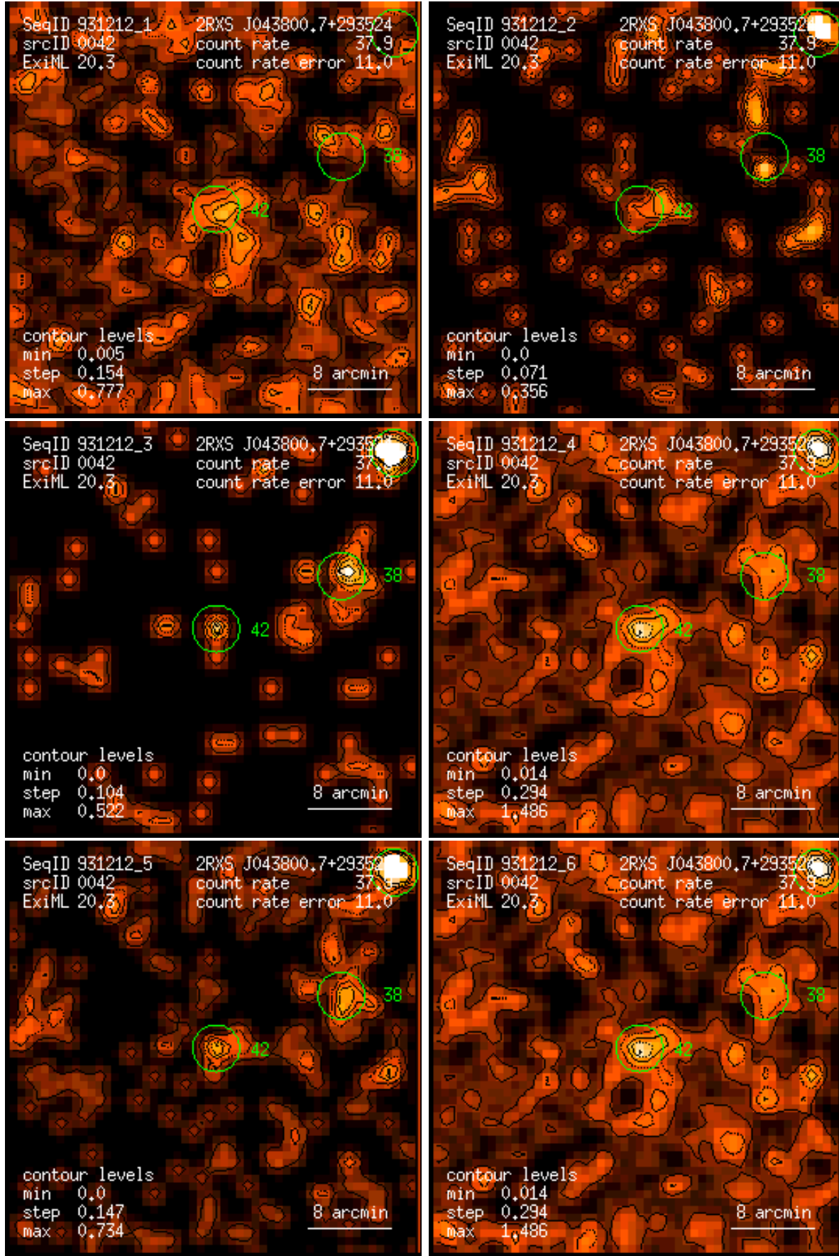
Figure 42: RASS 931212: detection 0042: band rate images, Gaussian filter: (1) PSPC channels 11 – 41, (2) 52 – 90, (3) 91 – 201, (4) 11 – 235, (5) 52 – 201, (6) 11 – 201. Broad band rates in counts/ks. Band rate contour levels in counts/ks/arcmin 2 .
