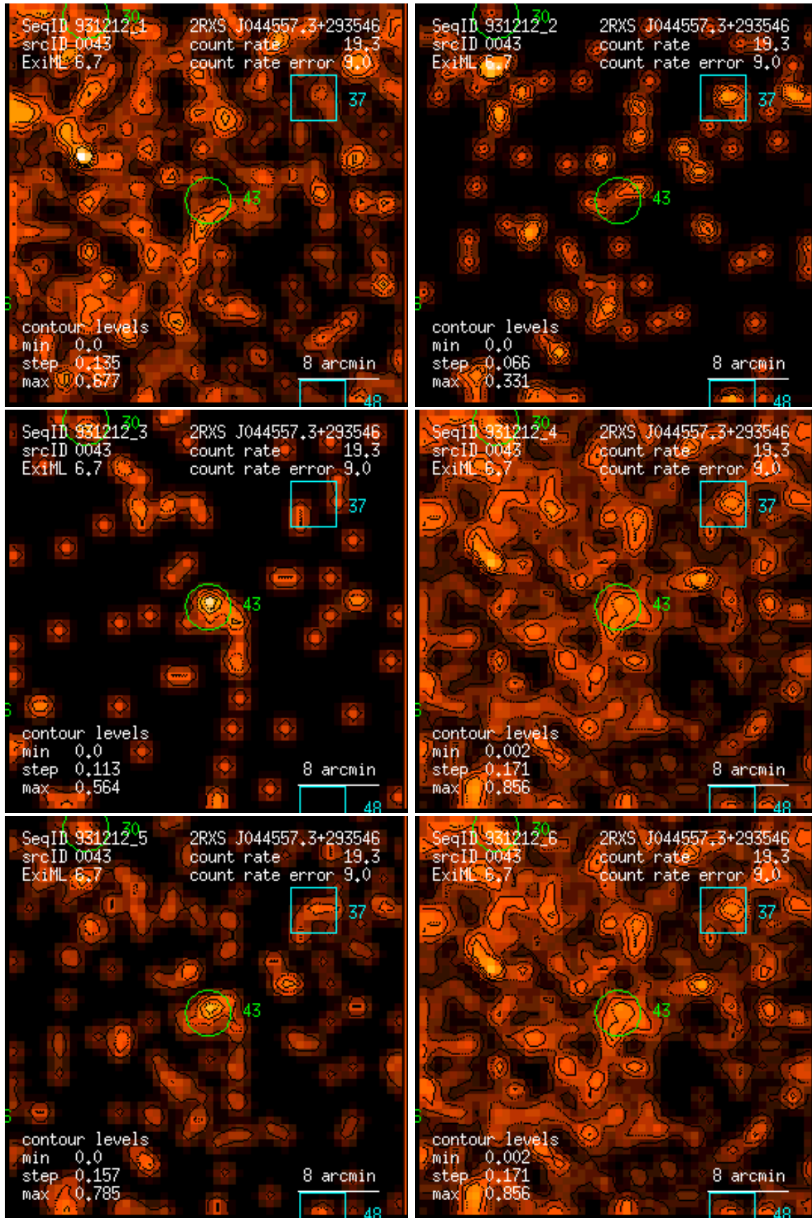
Figure 43: RASS 931212: detection 0043: band rate images, Gaussian filter: (1) PSPC channels 11 – 41, (2) 52 – 90, (3) 91 – 201, (4) 11 – 235, (5) 52 – 201, (6) 11 – 201. Broad band rates in counts/ks. Band rate contour levels in counts/ks/arcmin 2 .
