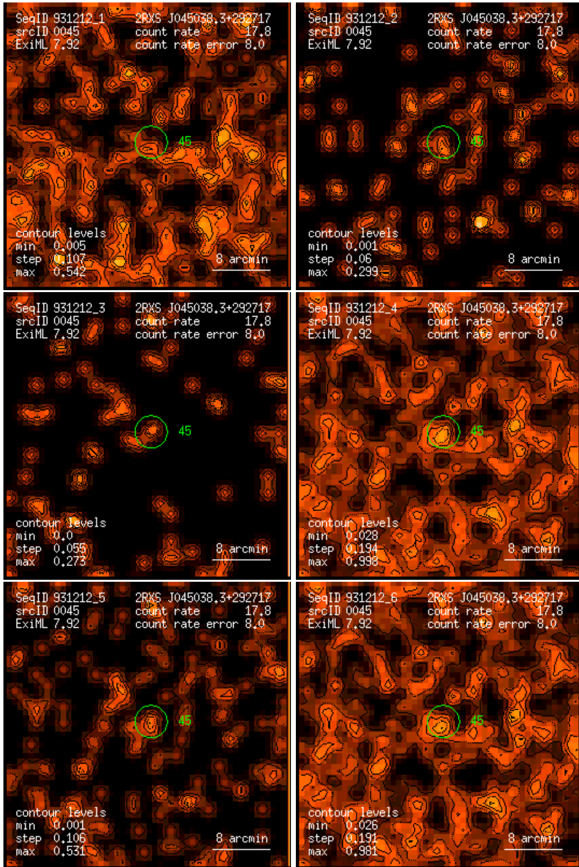
Figure 45: RASS 931212: detection 0045: band rate images, Gaussian filter: (1) PSPC channels 11 – 41, (2) 52 – 90, (3) 91 – 201, (4) 11 – 235, (5) 52 – 201, (6) 11 – 201. Broad band rates in counts/ks. Band rate contour levels in counts/ks/arcmin 2 .
