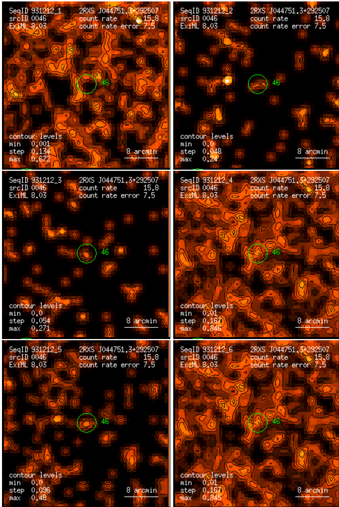
Figure 46: RASS 931212: detection 0046: band rate images, Gaussian filter: (1) PSPC channels 11 – 41, (2) 52 – 90, (3) 91 – 201, (4) 11 – 235, (5) 52 – 201, (6) 11 – 201. Broad band rates in counts/ks. Band rate contour levels in counts/ks/arcmin 2 .
