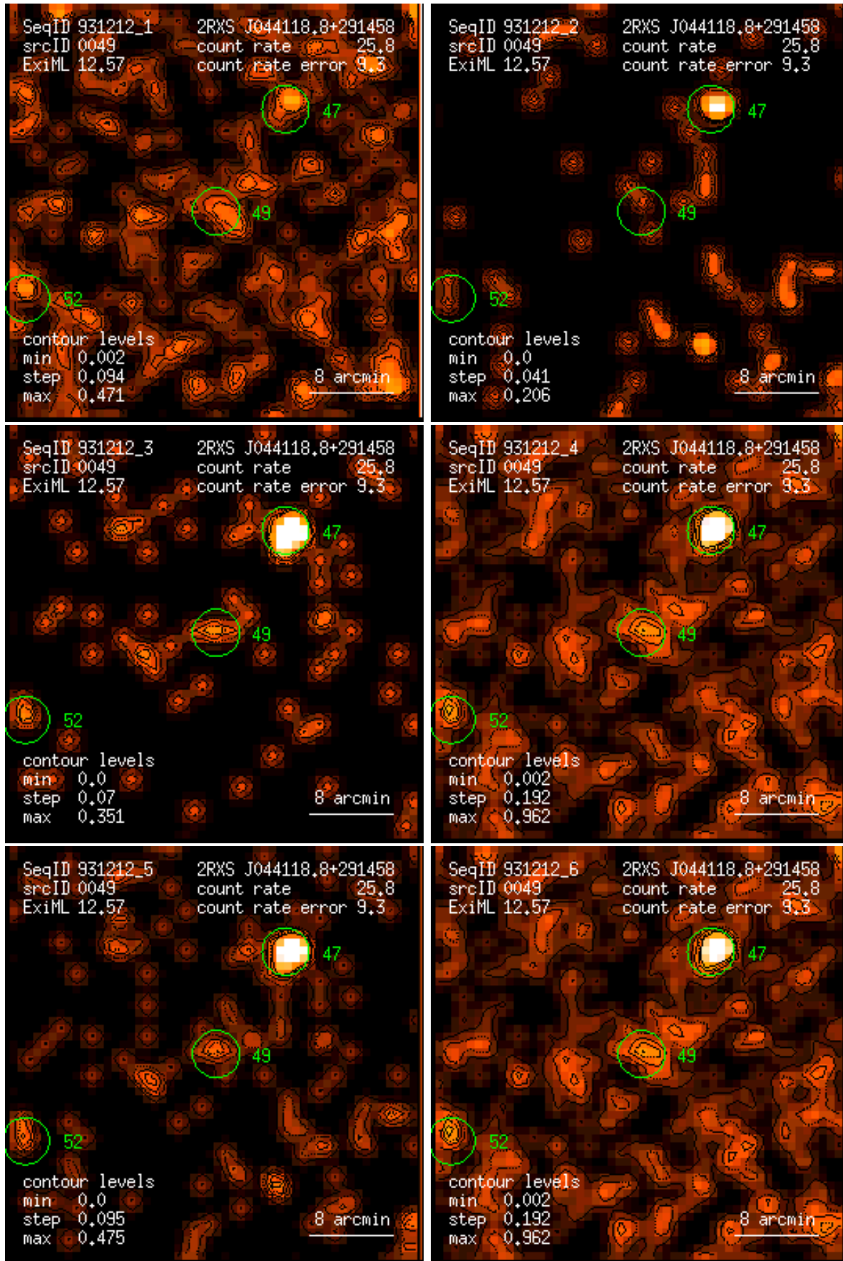
Figure 49: RASS 931212: detection 0049: band rate images, Gaussian filter: (1) PSPC channels 11 – 41, (2) 52 – 90, (3) 91 – 201, (4) 11 – 235, (5) 52 – 201, (6) 11 – 201. Broad band rates in counts/ks. Band rate contour levels in counts/ks/arcmin 2 .
