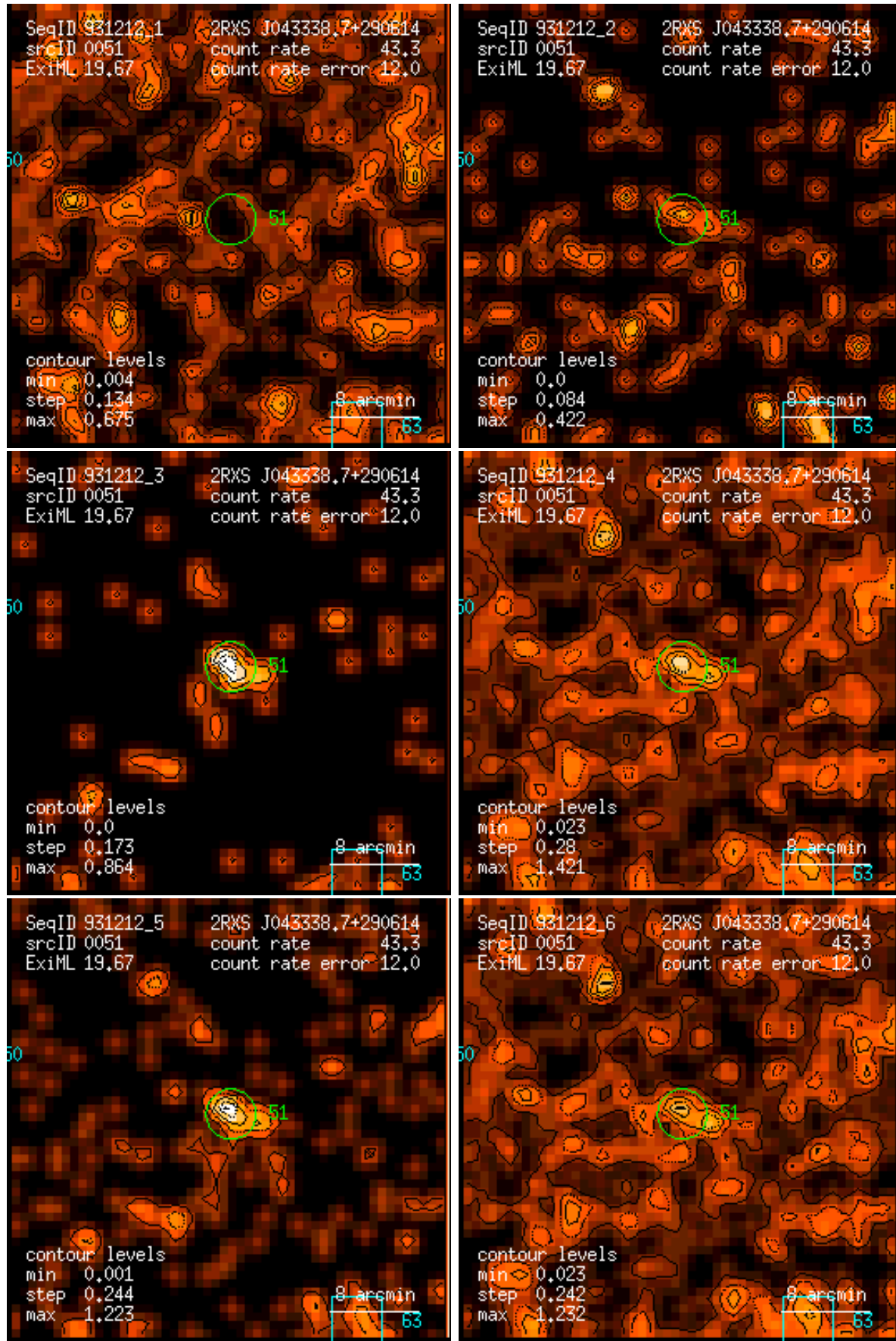
Figure 51: RASS 931212: detection 0051: band rate images, Gaussian filter: (1) PSPC channels 11 – 41, (2) 52 – 90, (3) 91 – 201, (4) 11 – 235, (5) 52 – 201, (6) 11 – 201. Broad band rates in counts/ks. Band rate contour levels in counts/ks/arcmin 2 .
