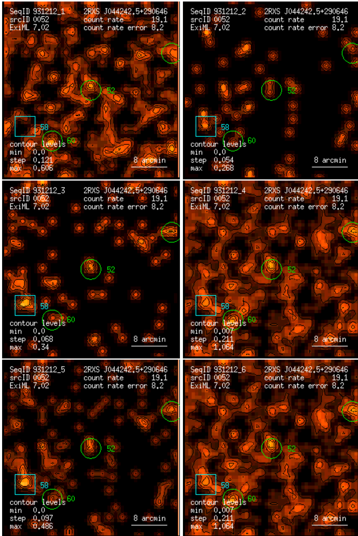
Figure 52: RASS 931212: detection 0052: band rate images, Gaussian filter: (1) PSPC channels 11 – 41, (2) 52 – 90, (3) 91 – 201, (4) 11 – 235, (5) 52 – 201, (6) 11 – 201. Broad band rates in counts/ks. Band rate contour levels in counts/ks/arcmin 2 .
