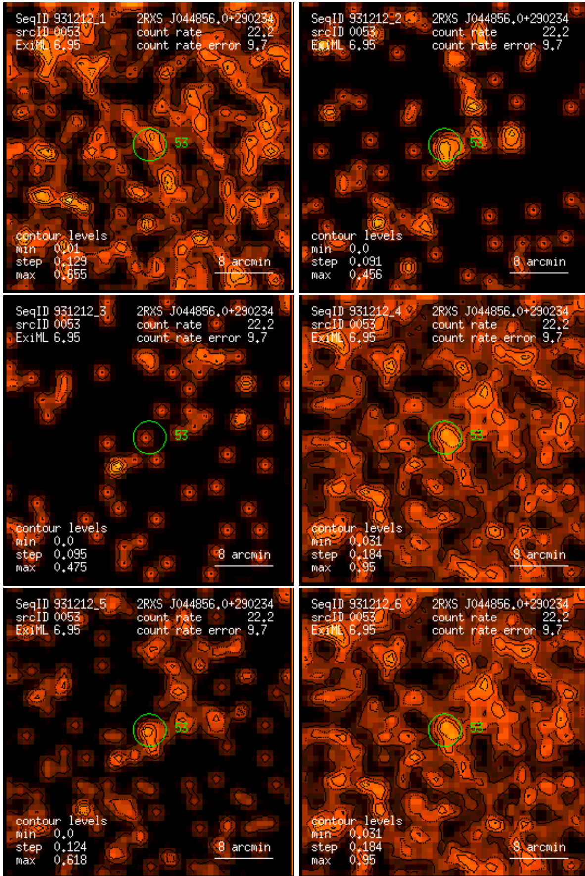
Figure 53: RASS 931212: detection 0053: band rate images, Gaussian filter: (1) PSPC channels 11 – 41, (2) 52 – 90, (3) 91 – 201, (4) 11 – 235, (5) 52 – 201, (6) 11 – 201. Broad band rates in counts/ks. Band rate contour levels in counts/ks/arcmin 2 .
