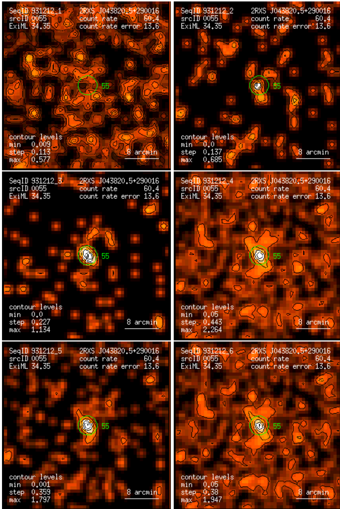
Figure 55: RASS 931212: detection 0055: band rate images, Gaussian filter: (1) PSPC channels 11 – 41, (2) 52 – 90, (3) 91 – 201, (4) 11 – 235, (5) 52 – 201, (6) 11 – 201. Broad band rates in counts/ks. Band rate contour levels in counts/ks/arcmin 2 .
