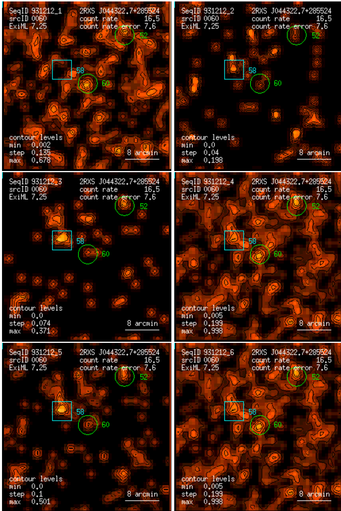
Figure 60: RASS 931212: detection 0060: band rate images, Gaussian filter: (1) PSPC channels 11 – 41, (2) 52 – 90, (3) 91 – 201, (4) 11 – 235, (5) 52 – 201, (6) 11 – 201. Broad band rates in counts/ks. Band rate contour levels in counts/ks/arcmin 2 .
